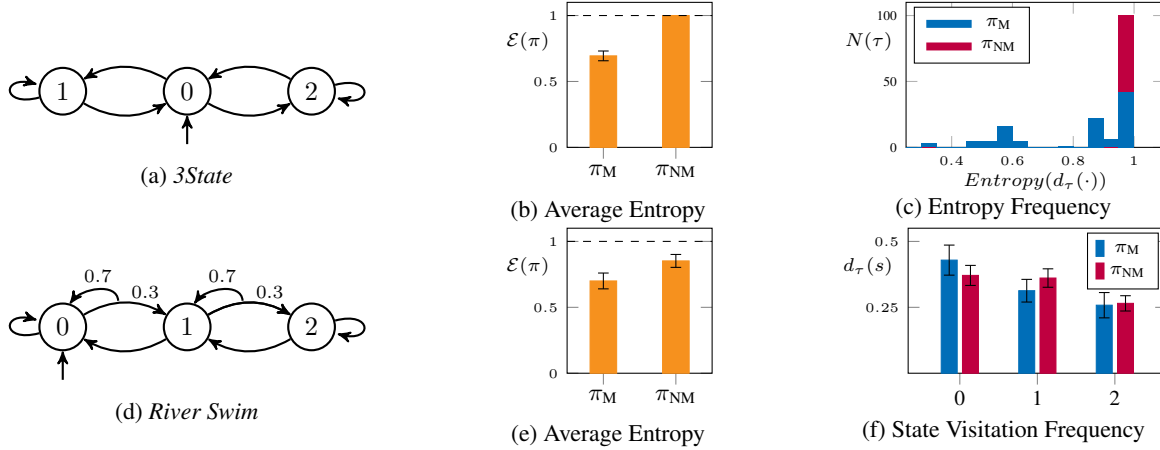
Figure 2. In (a, d), we illustrate the 3State and River Swim CPMs. Then, we report the average entropy induced by an optimal (stationary) Markovian policy \pi_M and an optimal non-Markovian policy \pi_{NM} in the 3State ( T = 9 ) (b) and the River Swim ( T = 10 ) (e). In (c) we report the entropy frequency in the 3State , in (f) the state visitation frequency in the River Swim . We provide 95% c.i. over 100 runs.
