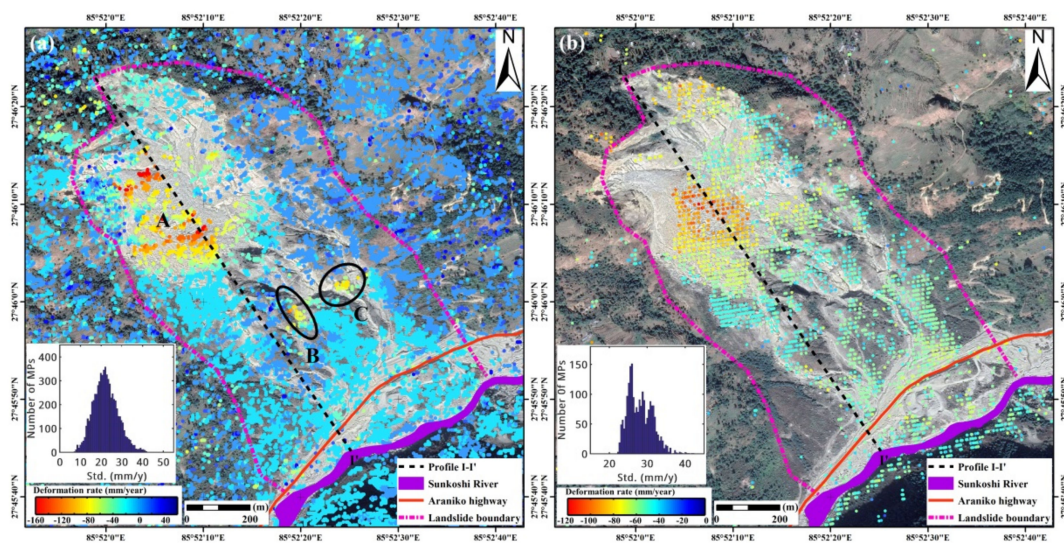
Figure 6. Post-disaster annual mean LOS deformation rate of Sunkoshi landslide measured by (a) ALOS-2 data during the period from September 2014 to October 2017, and (b) Sentinel-1 data during the period from January 2017 to October 2019. The repaired road and dredged river are also rendered. The subfigures on the lower-left corner show the histograms of standard deviation distribution of deformation rate.
