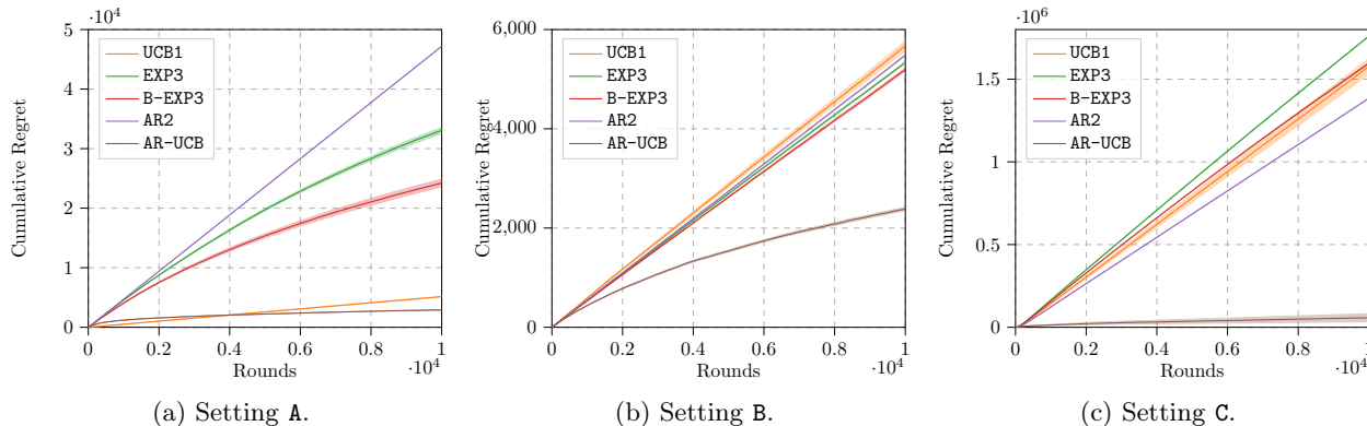
Figure 8: Cumulative regret of AR-UCB and the others bandit baselines in the case of k = 1 (100 runs, mean \pm std).
