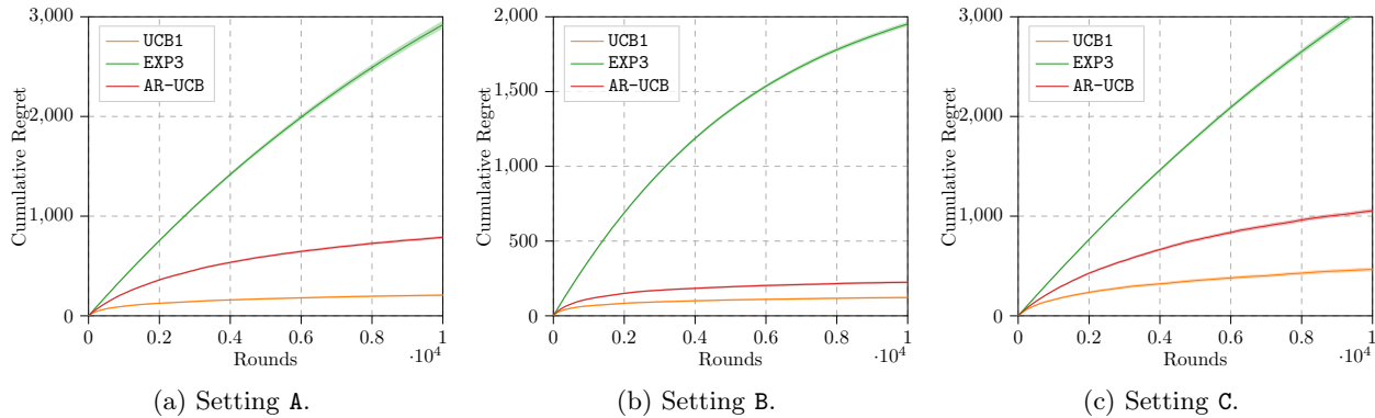
Figure 6: Cumulative regret of AR-UCB, UCB1, and EXP3 in the case of k = 0 (100 runs, mean \pm std).
