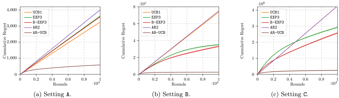
Figure 1: Settings and cumulative regret of AR-UCB and multiple baselines (100 runs, mean \pm std).
