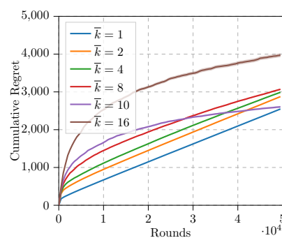
Figure 3: Effect of the choice of parameter \bar{k} on the AR-UCB cumulative regret (100 runs, mean \pm std).
