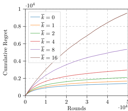
Figure 7: Cumulative regret of AR-UCB in the case of k = 0 , in with \bar{k} parameter misspecified (100 runs, mean \pm std).
