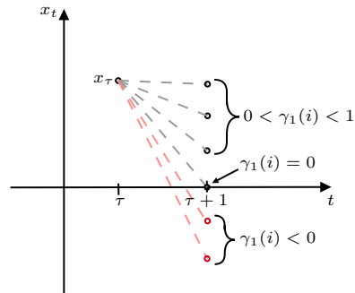
Figure 5: The effect of \gamma_1(a) in the evolution of the state x_t , in the case of a non-negative one (in black), and a negative one (in red).
