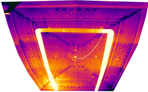
Figure 2. Thermal mosaic of one of the rooms with the vaulted brick ceiling.
