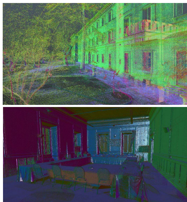
Figure 1. Perspective images of the point cloud from the exterior and internal spaces of the building.
