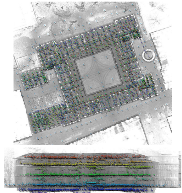
Figure 3. Top and lateral orthographic view of the complete aligned point cloud with individual scan points highlighted.
