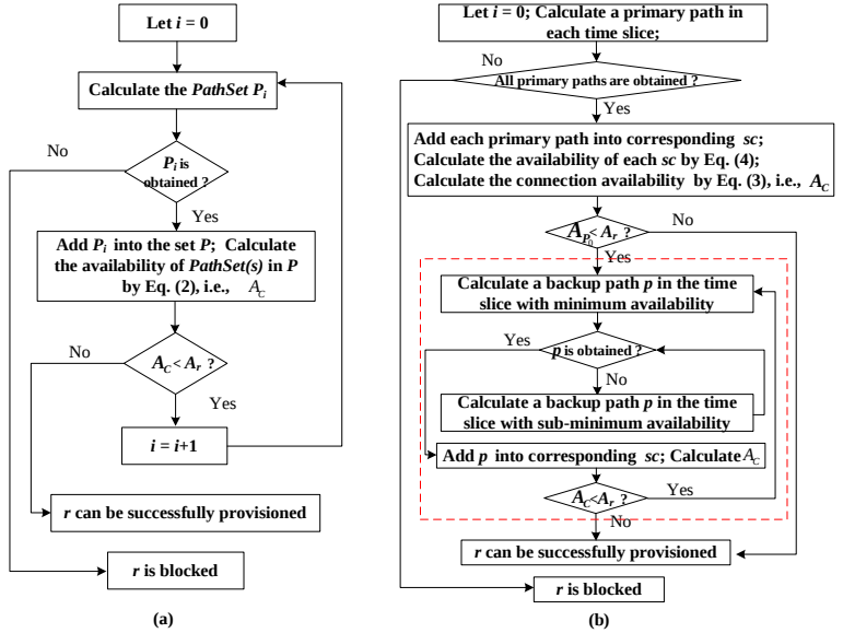
Fig. 2. (a) MP-ADP algorithm; (b) TS-ADP algorithm.
