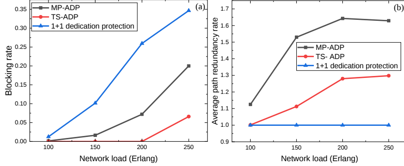
Fig. 4. Comparison for availability requirement 0.9999, (a) blocking rate, (b) APR.
