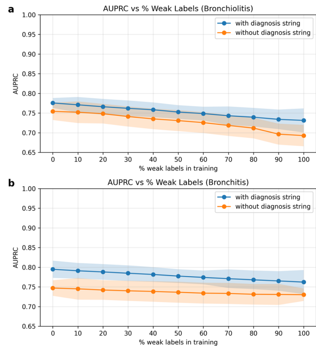
Fig. 4. AUPRC with varying percentages of weak labels on the bronchiolitis (a) and bronchitis (b) datasets. Mean AUPRC ( \pm 95\% CI) on gold labels, with and without diagnosis strings, as different proportions of gold labels are replaced by weak labels. Results are averaged over 5 repetitions of cross-validation. The y-axis is truncated to improve visibility of the trend.
