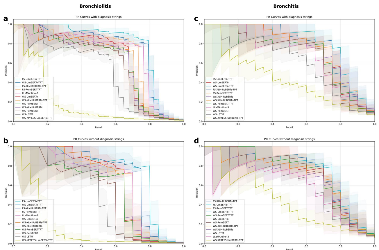
Fig. 3. Precision-Recall curves on the bronchiolitis (a, b) and bronchitis (c, d) gold labels with (a, c) and without (b, d) diagnosis strings. Shaded areas represent 95% C.I.
