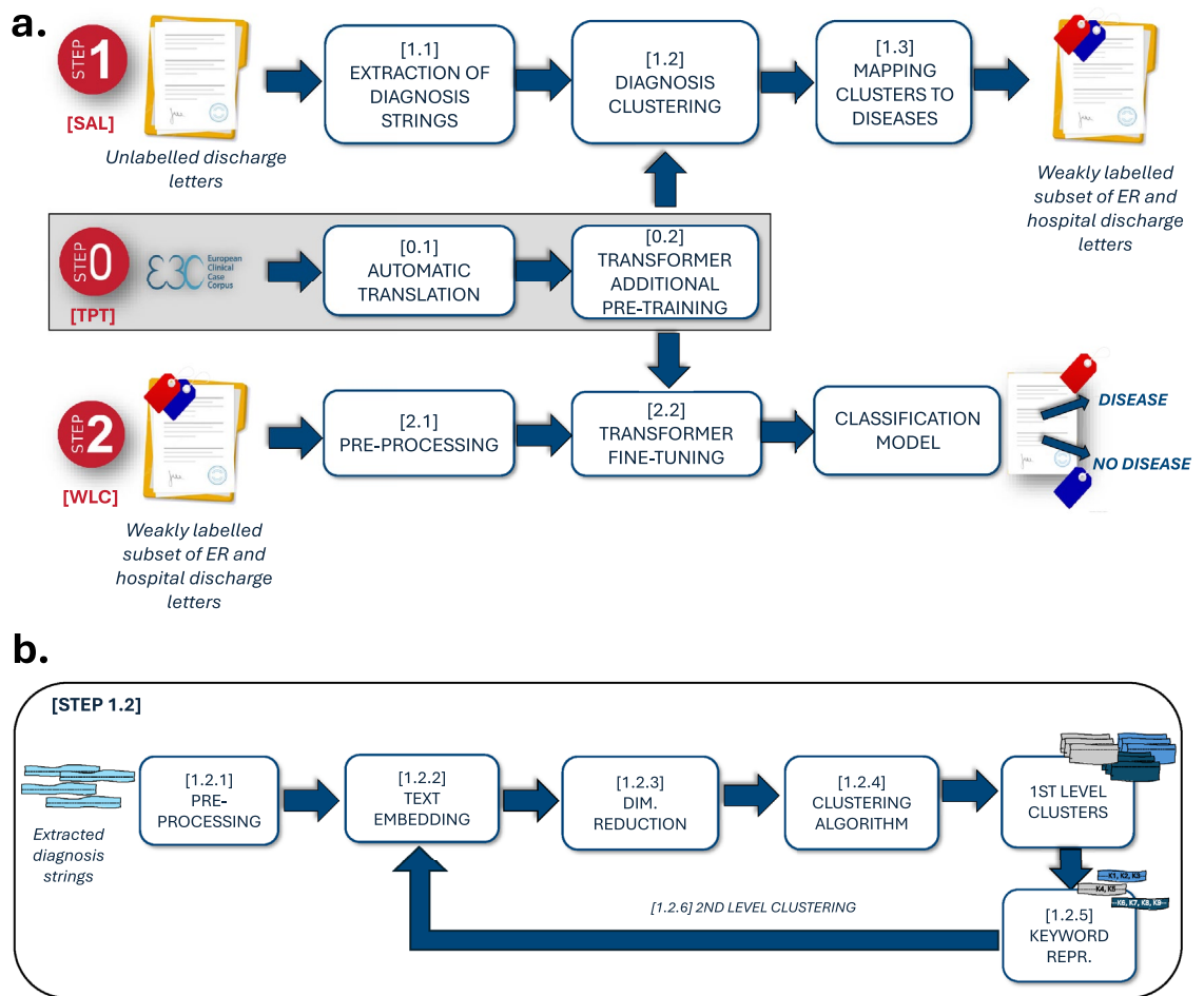
Fig. 1. (a) Diagram of the full pipeline for weakly supervised classification of discharge letters. Step 0 (TPT) consists in additional pre-training of a transformer-based model on a dataset of medical documents in Italian, including documents automatically translated into Italian. Step 1 (SAL) is the core of the pipeline, consisting in the automatic extraction of diagnosis strings from the letters, their clustering (exploiting the model from TPT) and the mapping of the clusters to the disease labels. This procedure leads to a weakly labelled subset of data that is used in Step 2 (WLC) to train a weakly supervised classification model. (b) Detailed diagram of the clustering step for diagnosis strings, corresponding to Step 1.2 of the full pipeline. The extracted diagnoses are embedded with a transformer-based model, and, after a dimensionality reduction step, clustered. Clusters are summarized with relevant keywords and the clustering is repeated on these clusters' representations.
