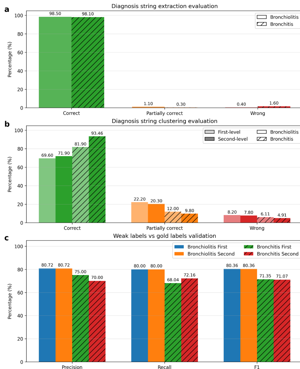
Fig. 2. Evaluation of the intermediate steps of the pipeline on the bronchiolitis and bronchitis datasets. a. Evaluation of diagnosis string extraction on 1,000 manually annotated diagnosis strings per dataset, reporting the percentage of extracted strings classified as correct, partially correct, or wrong. b. Evaluation of diagnosis clustering after first-level and second-level clustering on the same set of annotated diagnosis strings. c. Validation of weak labels against gold labels in terms of precision, recall, and F1-score, reported separately for labels obtained from first-level and second-level clustering.
