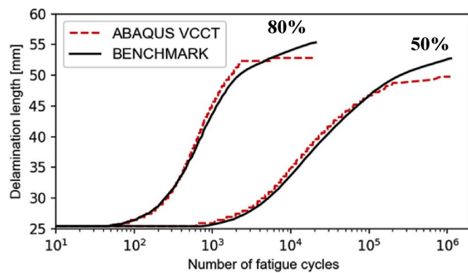
Fig. 15. Fatigue delamination propagation in MMB specimen.
