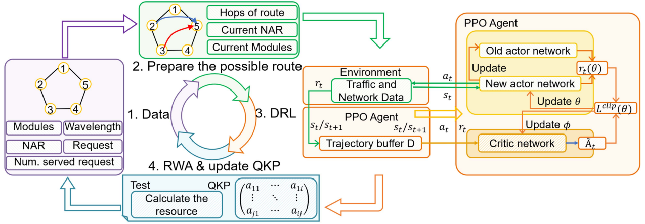
FIGURE 3. Operating mechanism of our proposed model.
