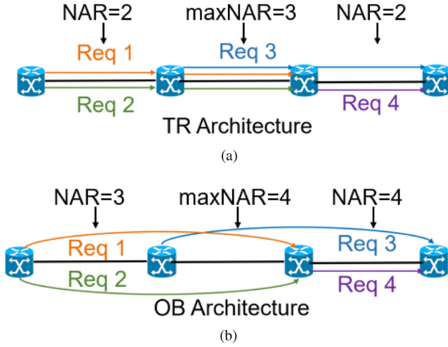
FIGURE 2. Example of NAR calculation. (a) NAR for TR, with \max\text{NAR}=3 . (b) NAR for OB, with \max\text{NAR}=4 .
