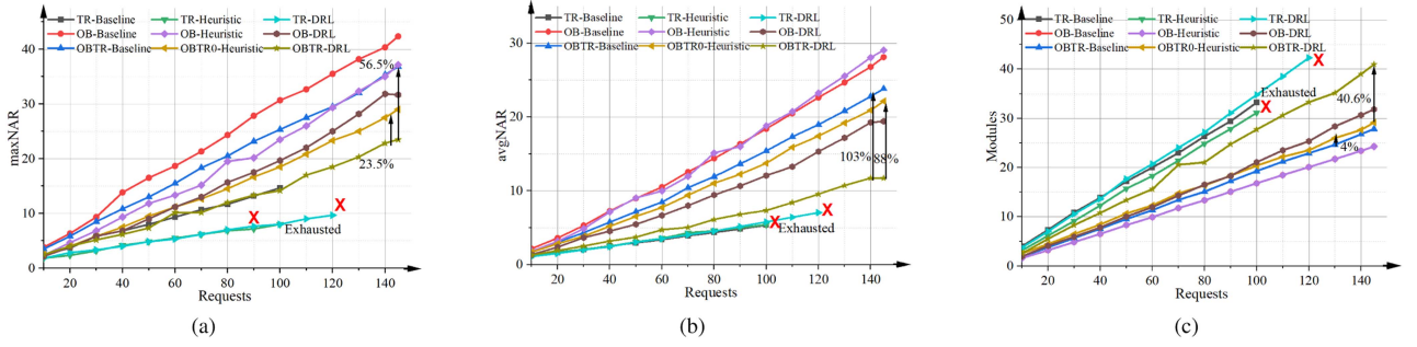
FIGURE 5. Evaluation of attack mitigation performance for three QKD architectures in the NSF topology. (a) maxNAR. (b) avgNAR. (c) Average number of used QKD modules per node.
