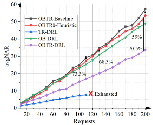
FIGURE 9. Evaluation of avgNAR for Mqn-20 topology.
