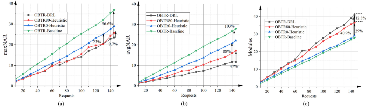
FIGURE 7. Attack mitigation performance of the proposed solution versus the heuristic for different \alpha values in the NSF topology. (a) maxNAR. (b) avgNAR. (c) Average number of used QKD modules per node.
