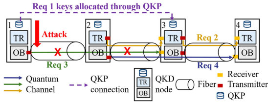
FIGURE 1. Example of technologies specific to QKD networks and the impact of a physical attack on a single optical fiber link.
