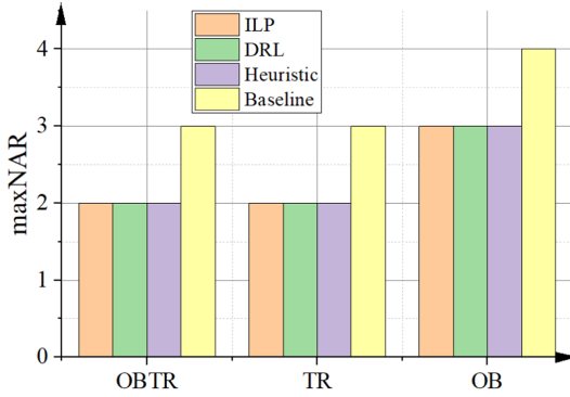
FIGURE 4. Evaluation for three QKD architectures in PoliQi topology.
