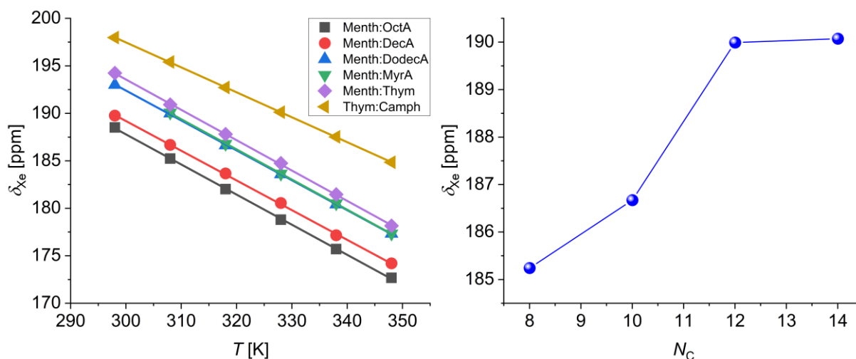
Figure 2. ^{129}\text{Xe} chemical shifts of xenon dissolved in EMs and DESs in the temperature range 298-348 K ( left panel ). The lines are linear fits to the data. Xenon chemical shift (308 K) vs carbon atom number ( right panel ).
