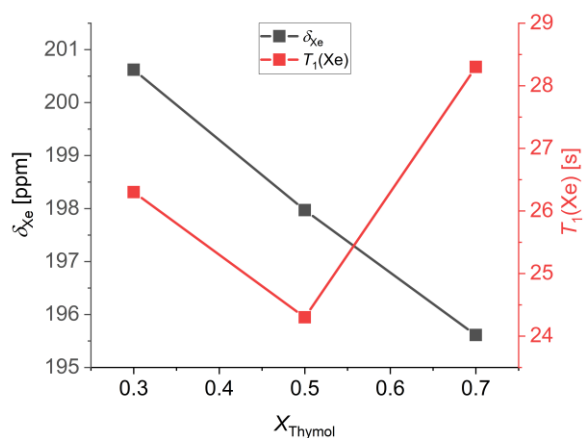
Figure 5. Chemical shift and T_1 relaxation times measured at 298 K of xenon dissolved in thymol:camphor mixtures as a function of the composition.
