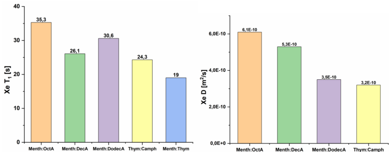
Figure 3. ^{129}\text{Xe} T_1 relaxation times and diffusion coefficients D , of xenon dissolved in ESs and DESs. All data are acquired at 298 K.
