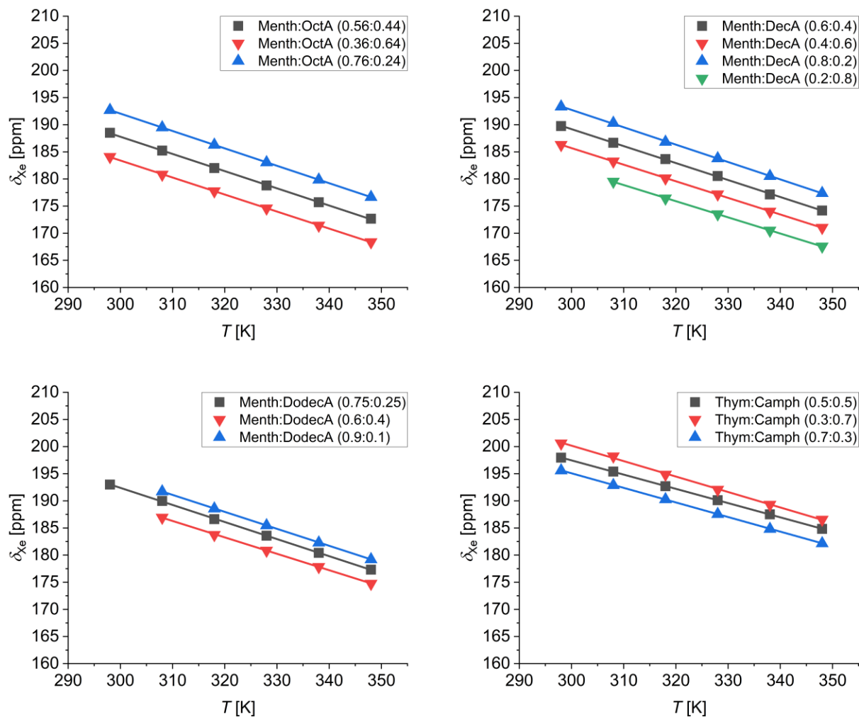
Figure 6. ^{129}\text{Xe} chemical shift as a function of temperature of xenon dissolved in the low-melting mixtures at different compositions.
