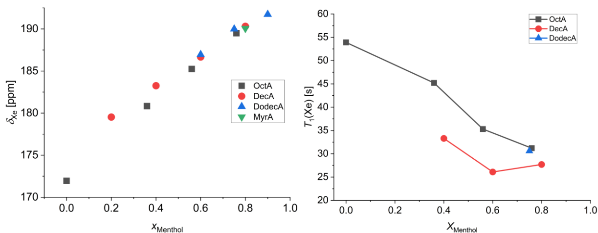
Figure 4. Chemical shifts measured at 308 K ( left ) and T_1 relaxation times measured at 298 K ( right ) of xenon dissolved in the low-melting mixtures as a function of the menthol molar fraction. The point at 0 menthol molar fraction refers to pure octanoic acid.
