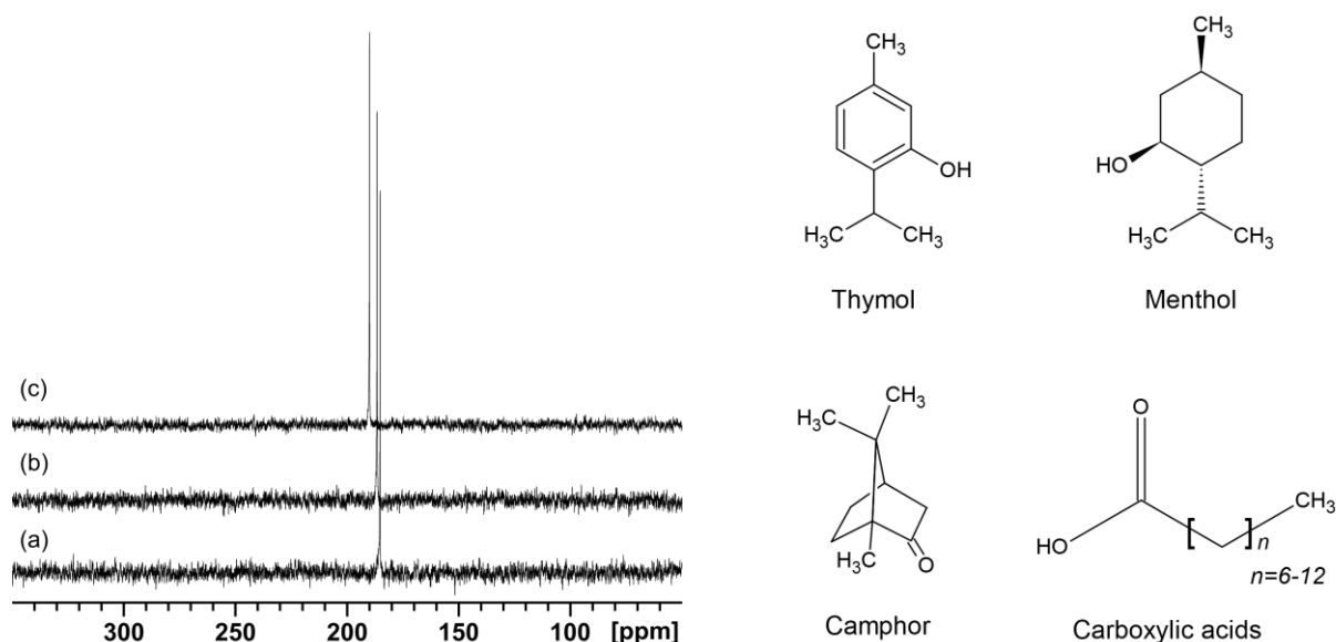
Figure 1. ^{129}\text{Xe} NMR spectra of xenon loaded in mixtures of menthol and octanoic (a), decanoic (b), and dodecanoic acid (c) at their eutectic composition, acquired at 298 K. Chemical structure of the EMs and DESs components.
