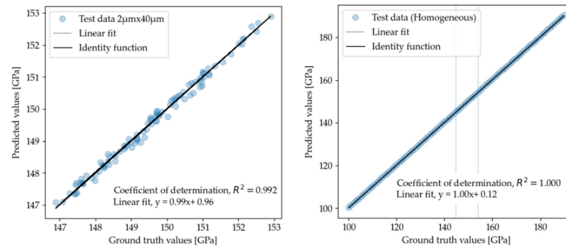
Figure 4. Performance of Model 2 on the test sets specified in Section 2.3.2.
