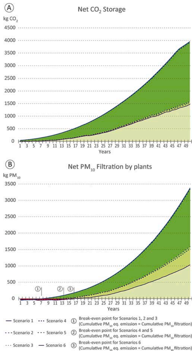
Fig. 13. A) Evolution over 50 years of net CO 2 storage of the urban forest considering the CO 2 eq. emissions in all the life cycle phases; B) Evolution over 50 years of cumulative net PM 10 filtration of the urban forest considering PM 10 eq. emissions in all the life cycle phases.
