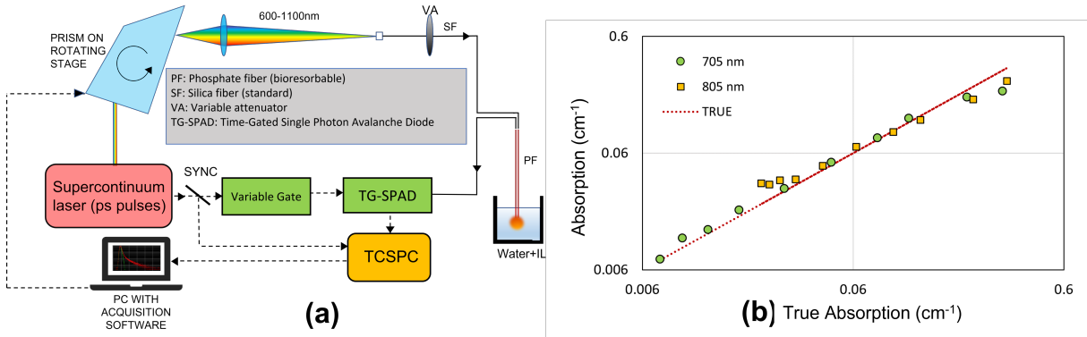
Figure 1. (a) Experimental setup; solid lines are optical paths and dashed lines are electronic paths; (b) absorption linearity using Intralipid phantoms
