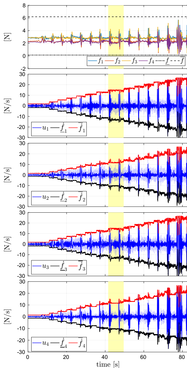
Fig. 10 Plots of the quadrotor tracking a discontinuous trajectory with steps in the position, while the controller limits are increased (the yellow region highlights the use of the identified ones). From top to bottom, the actuator forces and their derivatives. In particular, all the signals remain inside the feasible region delimited by the constraints
