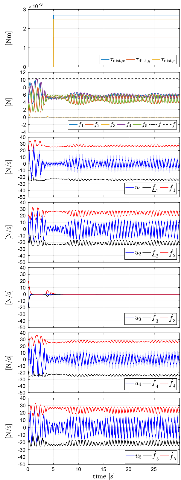
Fig. 21 Plots of the Tilt-Hex with rotor failure and \beta = 0 deg while hovering. The robot is disturbed with a constant external torque \tau_{\text{dist}} , activated at t = t_1 . From top to bottom, the disturbance torque, the actuator forces and their derivatives. In particular, all the signals remain inside the feasible region delimited by the constraints
