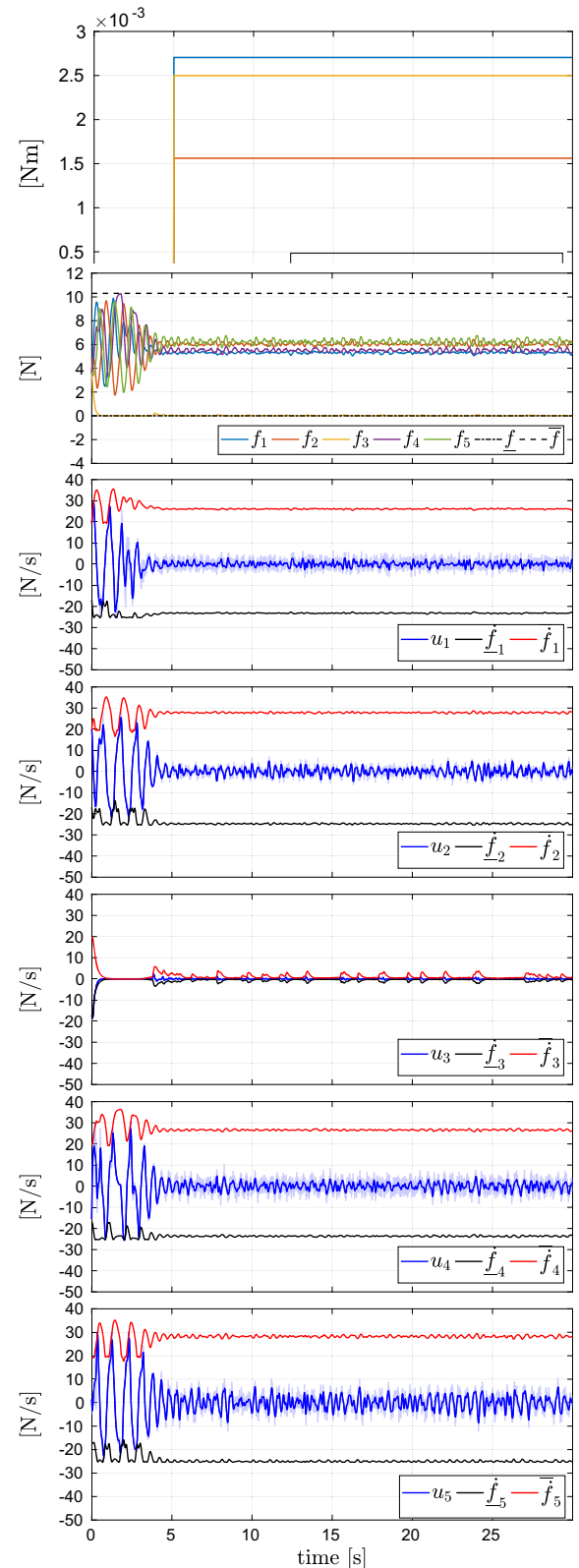
Fig. 23 Plots of the Tilt-Hex with rotor failure and \beta = -25 deg while hovering. The robot is disturbed with a constant external torque \tau_{dist} , activated at t = t_1 . From top to bottom, the disturbance torque, the actuator forces and their derivatives. In particular, all the signals remain inside the feasible region delimited by the constraints
