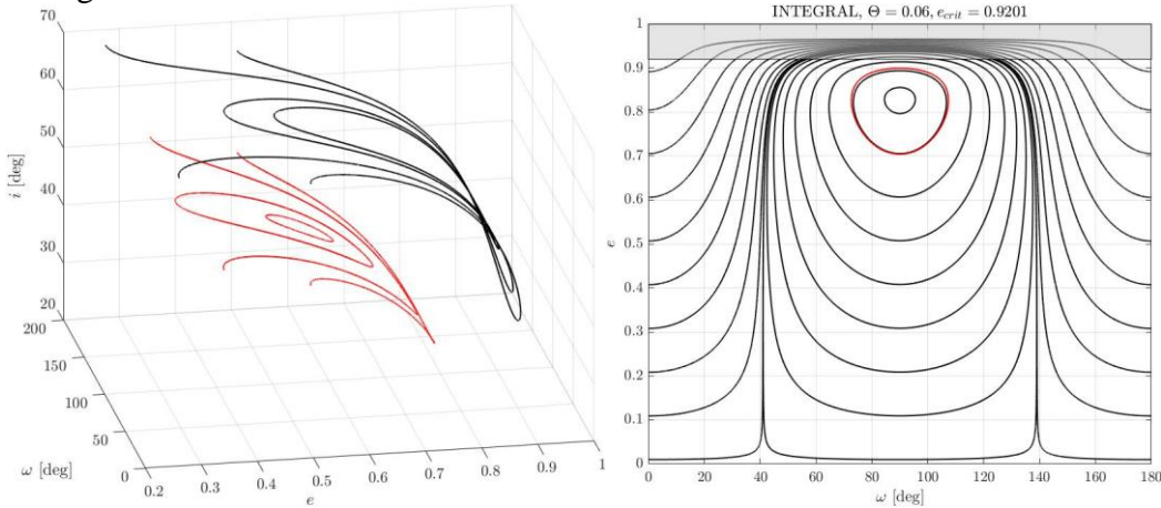
Fig 1 Left: Phase space map, lunar perturbation only, red line: \Theta = 0.3 , black line: \Theta = 0.1 ; Right: Phase space portrait of the INTEGRAL mission, \Theta = 0.06, e_{crit} = 0.9201 , red curve: initial phase curve of the INTEGRAL mission.
