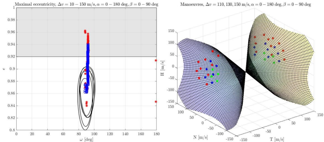
Fig 2 Left: Result of grid search shown in e, \omega phase space, black curve: initial phase curve, blue markers: e_{max} for successful re-entries, red markers: e_{max} for non-successful re-entries, grey zone: e_{max} > e_{crit} ; Right: Demonstration of manoeuvres corresponding to successful re-entries.
