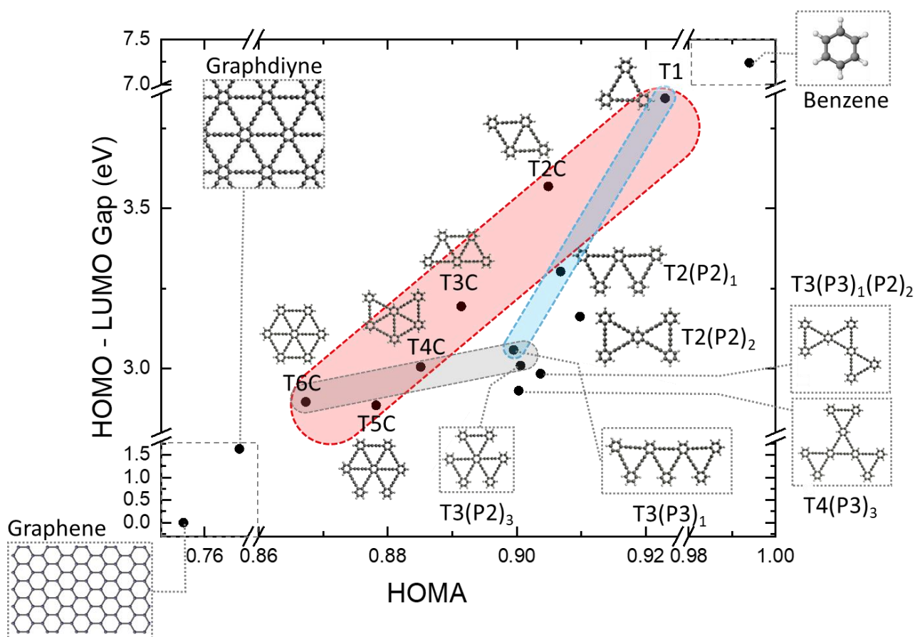
Figure 3: Correlation between computed HOMO-LUMO gaps (in eV) and mean HOMA values of some of the 2D-GDY fragments investigated (see Table S1). Shaded areas show some peculiar trends discussed in the text. Graphene and benzene are reported as a reference. See the methods section for a definition of the HOMA parameter.
