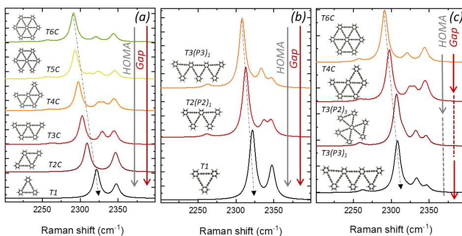
Figure 4: DFT-computed Raman spectra of 2D-GDY molecular fragments for different subgroups of structures. The corresponding trend of HOMA and gap is represented by arrows (dotted line indicates no substantial variation).
