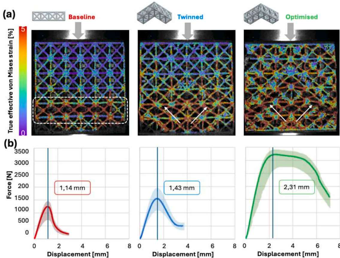
Fig. 6. Experimental compression response of baseline , twinned , and optimized lattice architectures. (a) Digital Image Correlation (DIC) maps in correspondence of the maximum load of the three classes during uniaxial compression, showing the spatial distribution of true effective von Mises strain (%) at comparable deformation states. (b) Corresponding force–displacement curves obtained from compression tests for the three architectures until fracture. The reported displacement values are corrected for machine compliance. Solid lines represent the mean response, while shaded regions indicate standard deviations. Rectangles highlight the displacement at peak load, illustrating the progressive increase in both peak force and deformation capacity from baseline to twinned and optimized designs. The compression direction is vertical in all specimens (grey arrow). For the twinned and optimized architectures, the twin boundary acts as a symmetry plane governing the observed deformation and shear-band development.
