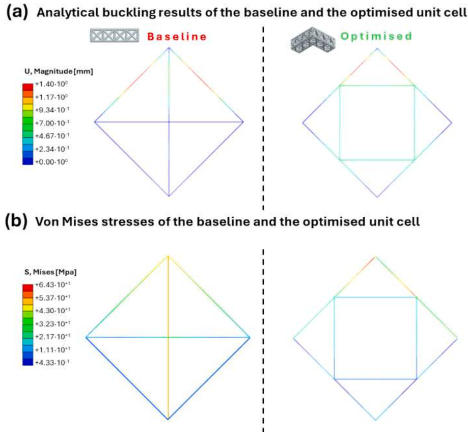
Fig. 3. Buckling and stress-based failure assessment of the baseline and optimized unit-cell frame models. (a) Linear perturbation buckling analysis of the Baseline (left) and Optimized (right) unit cells, reported as the first-mode buckling shapes and corresponding load multipliers. (b) Von Mises stress fields [MPa] computed by applying to each unit cell its respective buckling load.
