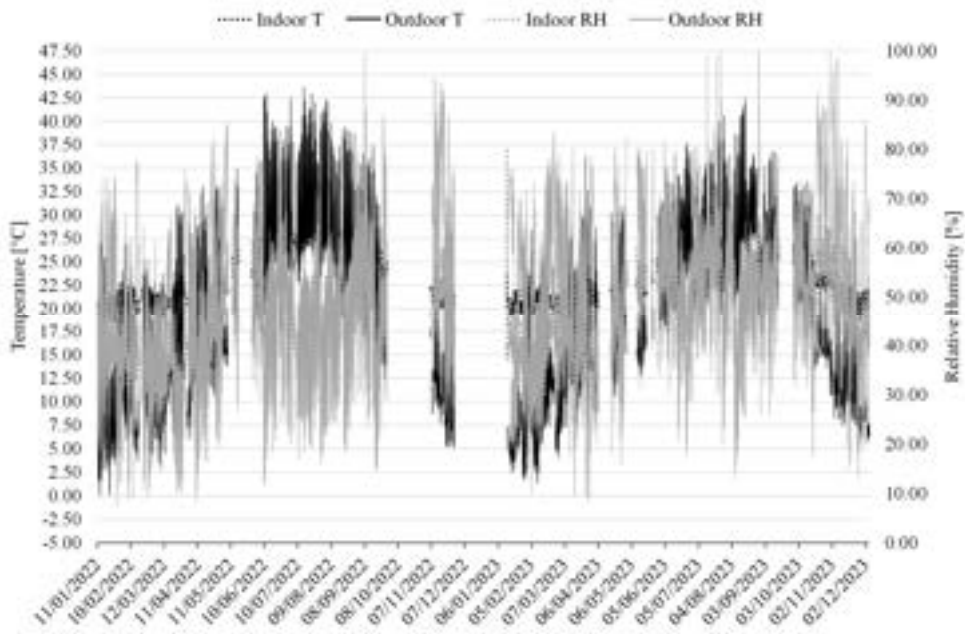
Fig. 7. Italian case study, temperature/humidity over time graph. The heating period indoor and outdoor mean temperatures are respectively equal to 21.26°C and 12.63°C, while the cooling period indoor and outdoor mean temperatures are respectively equal to 26.76°C and 26.55°C. Authors' elaboration.
