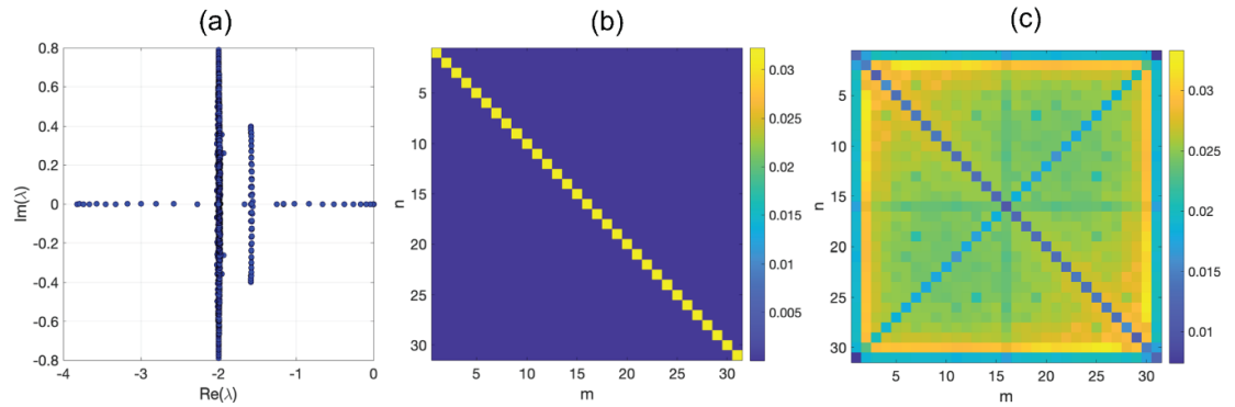
Figure 3. Same as figure 2, but for h = 0 (reciprocal and disorder-free model). Note the disappearance of the LSE.
