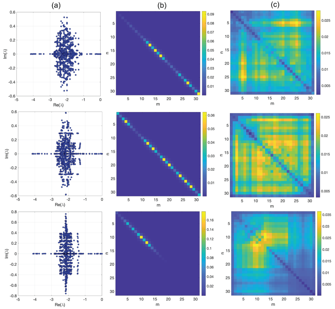
Figure 4. Same as figure 2, but in the stochastic lattice where h_n can take only the two values h_n = \pm h with the same probability. Parameter values are as in figure 2 ( J = 0.2 , Q = 1 , h = 0.4 and L = 31 ). The three row in the figures refer to three realizations of the stochastic sequence \{h_n\} .
