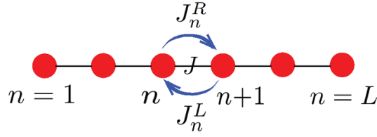
Figure 1. Schematic a tight-binding lattice made of L sites with coherent ( J ) and site-dependent asymmetric incoherent ( J_n^R, J_n^L ) hopping between adjacent sites. Open boundary conditions are assumed. The incoherent hopping rates are given by J_n^L = Q \exp(h_n) and J_n^R = Q \exp(-h_n) , where h_n is the asymmetry parameter. For h_n = h \neq 0 , the model displays the LSE. When h_n are independent stochastic variables that can assume only the two values +h or -h with the same probability, the system is globally reciprocal and the LSE disappears. Instead, erratic Liouvillian skin localization is observed, associated to sub-diffusive spreading of an initially-localized boson in the lattice bulk.
