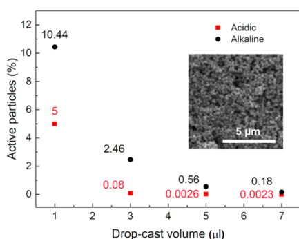
Figure 5. Percentage of electroactive particles as a function of drop-cast volume on GC electrode under acidic ( \text{H}_2\text{SO}_4 , pH 4.5, room temperature) (red) and alkaline (NaOH, pH 12.8, room temperature) (black) conditions. The inset shows the SEM micrograph of 7 \mu\text{L} of concentrated solution drop-cast on the GC electrode. Scale bar: 5 \mu\text{m} .
