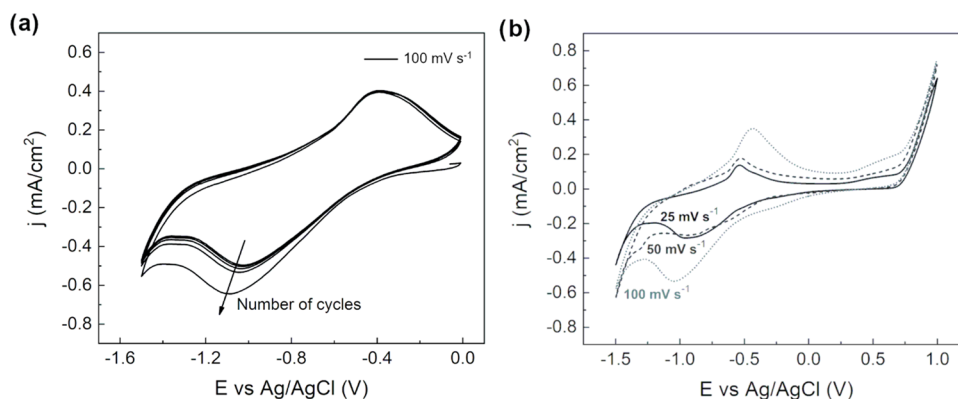
Figure 4. (a) Cyclic voltammetry ( 100 \text{ mV s}^{-1} ) at room temperature of magnetite nanoaggregates under alkaline conditions (NaOH, pH 12.8, room temperature). (b) Cyclic voltammetry ( 25, 50, 100 \text{ mV s}^{-1} ) at room temperature of magnetite particles under alkaline conditions (NaOH, pH 12.8, room temperature). Supported electrode configuration.
