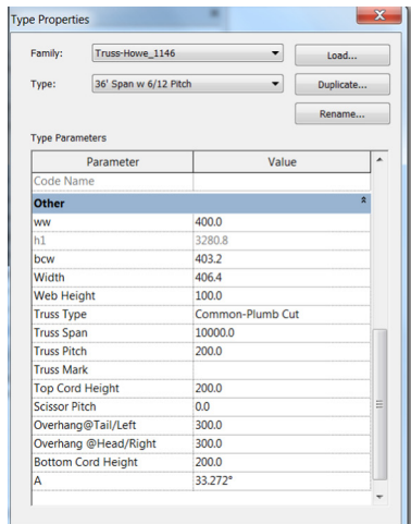
Fig. 1. In parametric modeling a database is associated to the different elements of the objects: the elements of the truss can be modified by changing the numerical values in the table.
