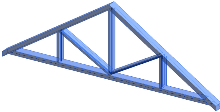
Fig. 1. In parametric modeling a database is associated to the different elements of the objects: the elements of the truss can be modified by changing the numerical values in the table.
