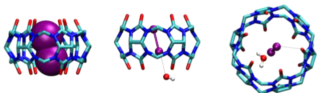
Figure 97. Stick-style views of the single-crystal X-ray structure of the cucurbit[6]uril–I 2 complex. Encapsulated diiodine, in space-filling style (left), is halogen-bonded with a water molecule (middle) and is bound to the carbonyl oxygen at the upper portal (right).
