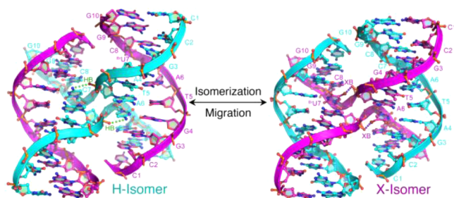
Figure 119. Competition between hydrogen-bonded (cyan strand) and halogen-bonded (magenta strand) structures in a four-stranded DNA junction. Reprinted with permission from ref 885. Copyright 2015 Springer.
