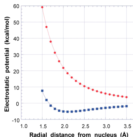
Figure 25. Computed electrostatic potential, B3PW91/6-311G(3d), of the chlorine atom in its valence state, 3s^23p_x^23p_y^23p_z^1 , as a function of the radial distance from the nucleus. The upper and red curve corresponds to the z-axis, the lower and blue curve to the x- and y-axes. In this valence state, V(r) is still positive at all radial distances along the z-axis, corresponding to the half-filled p_z orbital. Along the x- and y-axes, however, V(r) is positive near the nucleus but then becomes negative, reflecting the doubly occupied p_x and p_y orbitals. Reprinted with permission from ref 26. Copyright 2010 Royal Society of Chemistry.
