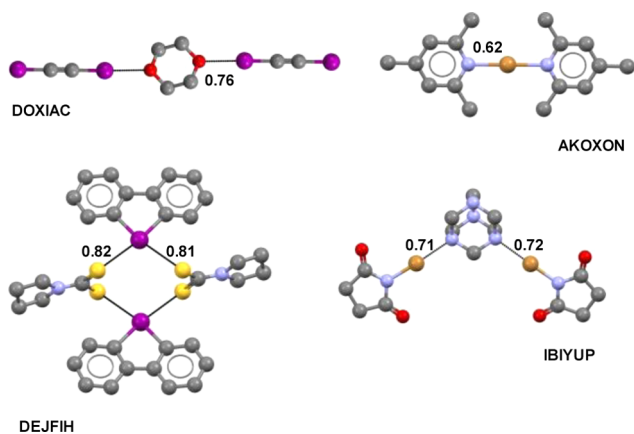
Figure 56. Representation of halogen-bonded crystal structures involving highly polarized halogen atoms. Hydrogen atoms are omitted for clarity. Color code: carbon, gray; nitrogen, blue; oxygen, red; iodine, purple; bromine, light brown; sulfur, dark yellow. XBs are dotted black lines. CSD Refcodes are reported: DOXIAC, 1,4-dioxane and diiodoacetylene; AKOXON, bis(2,4,6-collidine)bromonium perchlorate; DEJFIH, dibenziodolyl pyrrolidinedithiocarbamate; IBYUP, hexamethylenetetramine and N -bromosuccinimide.
