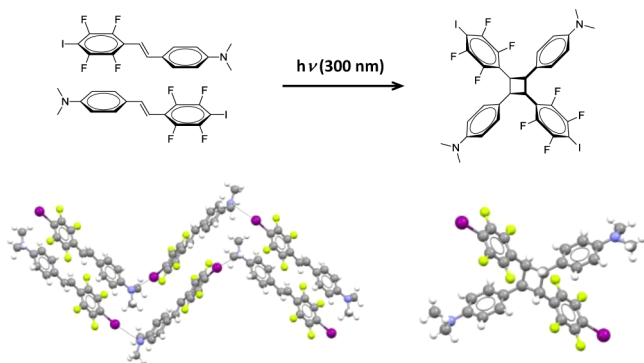
Figure 104. Top: schematic representation of the solid-state photoreaction of an XB-based self-complementary tecton to yield a tetratopic self-complementary cyclobutane derivative. Bottom: views of the crystal packing of two infinite and halogen-bonded chains formed in the solid state by the starting olefin (left, XBs as dotted black lines), and of the cyclobutane derivative obtained after UV irradiation (right). Color code: carbon, gray; nitrogen, blue; iodine, purple; fluorine, yellow; hydrogen, white. XBs are dotted black lines.
