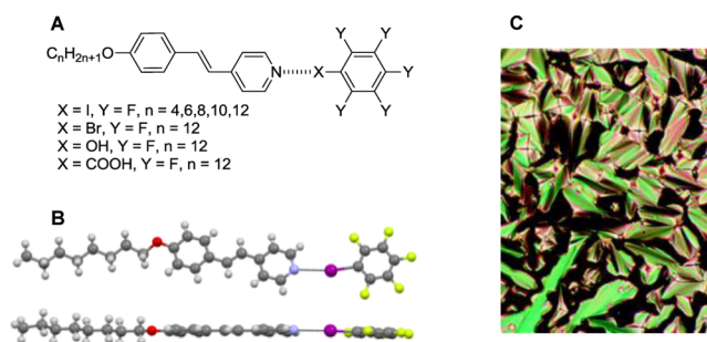
Figure 106. (A) Chemical structures of the halogen-bonded LCs reported in ref 837 and corresponding hydrogen-bonded analogues. (B) Crystal structure of the (octyloxy)stilbazole/iodopentafluorobenzene dimer evidencing the presence of I...N XB (shown as black dotted lines) and the coplanarity of the aromatic rings. Color code: gray, carbon; yellow, fluorine; purple, iodine; sky blue, nitrogen; white, hydrogen. (C) Polarized optical micrograph of the smectic A texture of the (hexyloxy)stilbazole/iodopentafluorobenzene dimer at 69° upon cooling. Reprinted from ref 837. Copyright 2004 American Chemical Society.
