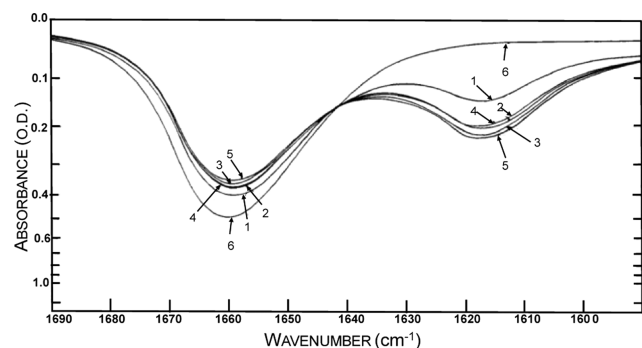
Figure 41. Infrared spectrum of the dimethylacetamide/iodine complex. As the \text{I}_2 concentration increases, the intensity of the free amide peak (1662 \text{cm}^{-1} ) decreases, while the intensity of the complex peak (1619 \text{cm}^{-1} ) increases. Reprinted from ref 394. Copyright 1960 American Chemical Society.
