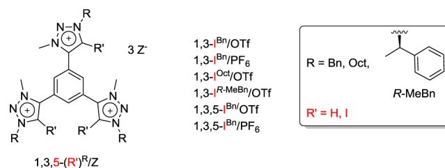
Figure 132. Bi- and tridentate polycationic XB donors based on the 5-iodo-1,2,3-triazolium synthon.
