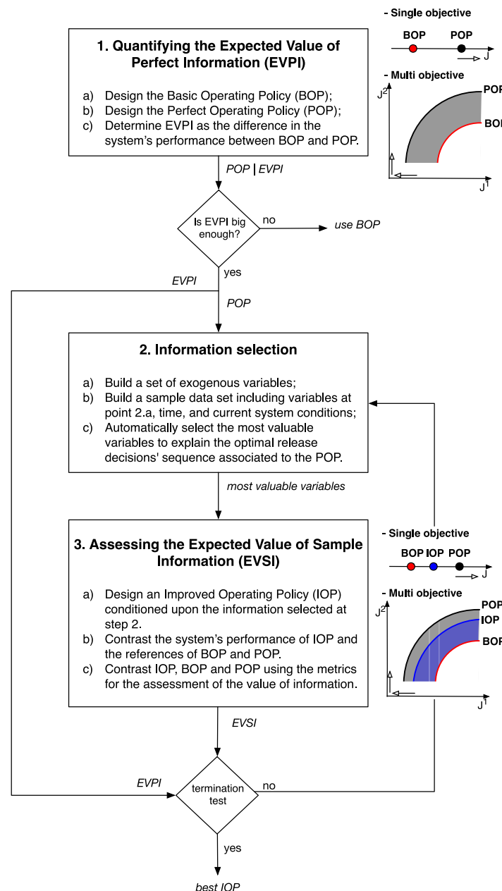
Figure 1. Schematization of the Information Selection and Assessment (ISA) framework.
