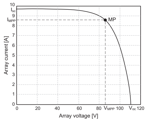
Fig. 1. Photovoltaic (PV) array characteristic curve.
