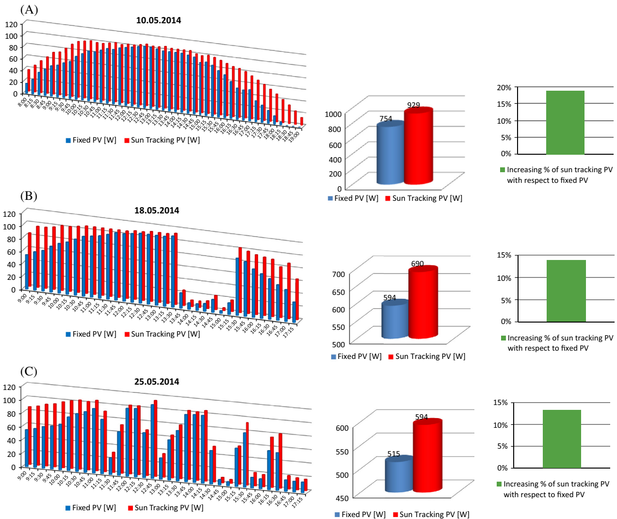
Fig. 8. Output power evaluated in different conditions: (a) clear sky, (b) partially clear sky, and (c) cloudy sky.
