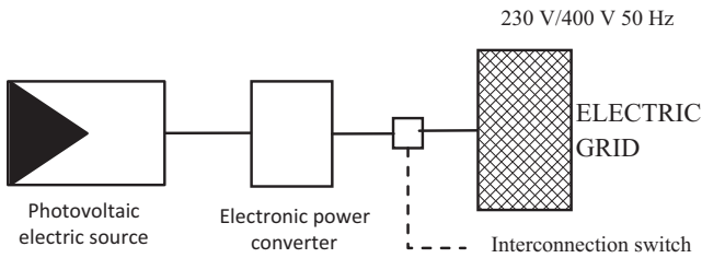
Fig. 3. PV electrical power system configuration.
