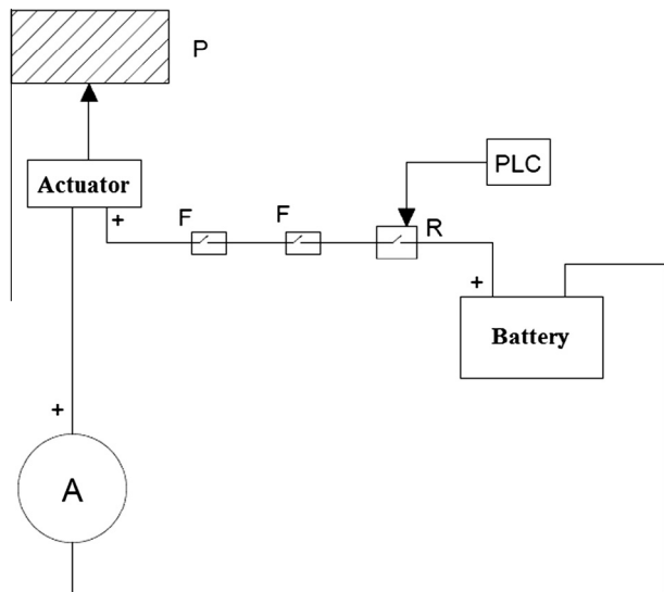
Fig. 6. Measuring circuit of the implemented sun-tracking PV power system.
