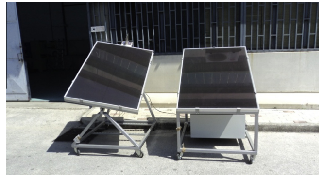
Fig. 5. Sun-tracking and fixed PV test systems.
