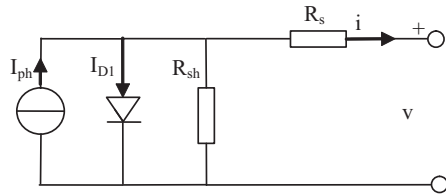
Fig. 2. Photovoltaic (PV) equivalent circuit.
