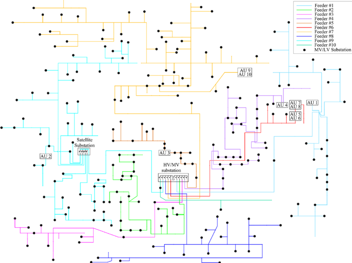
Figure 1. The MV distribution network (20 kV) involved in the Project.
