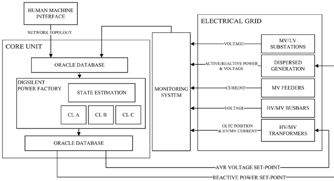
Figure 12. Data exchanged to perform the voltage control on the MV network.
