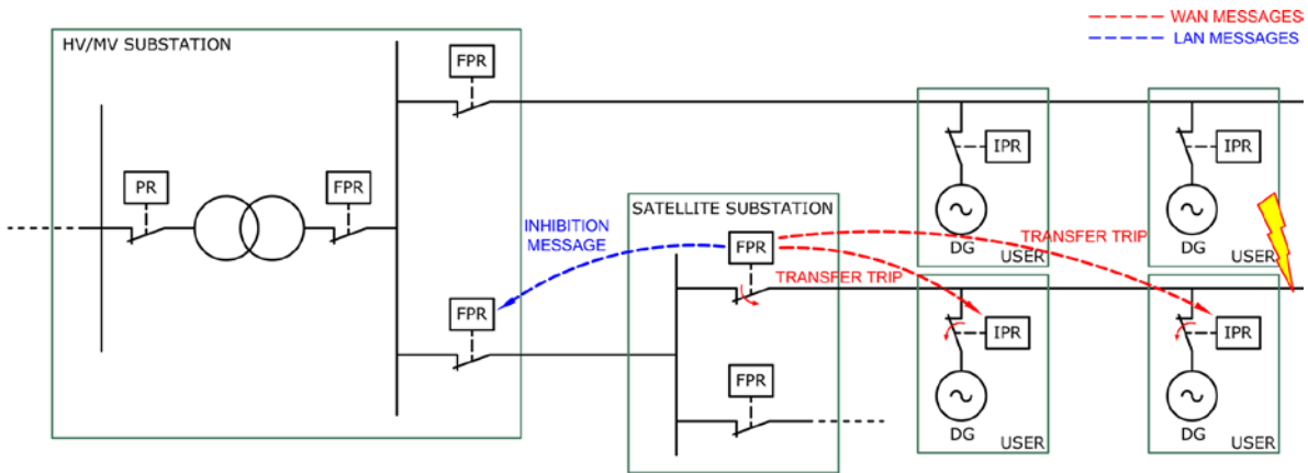
Figure 9. Automatic reclosing with logic selectivity.
