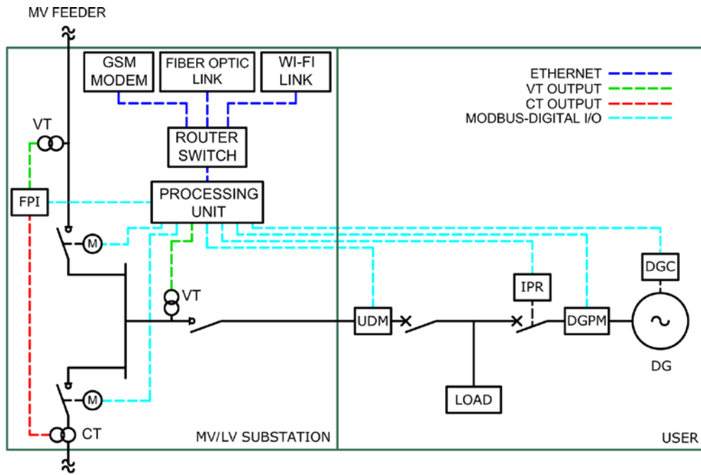
Figure 5. Functional architecture of the system for Active Users.
