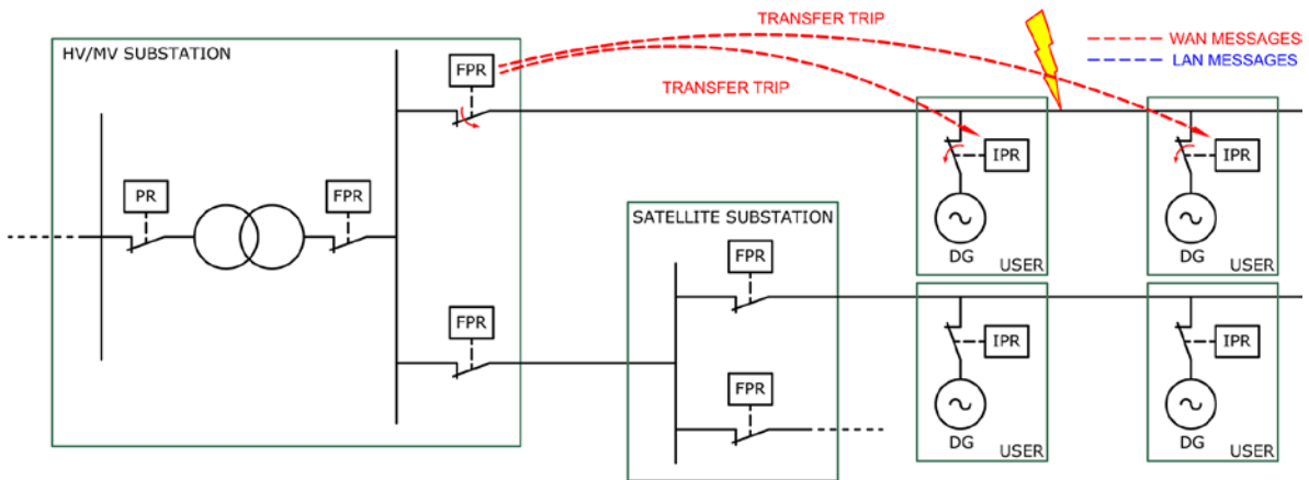
Figure 6. Transfer trip message sent to the DG units underlying a distribution feeder.
