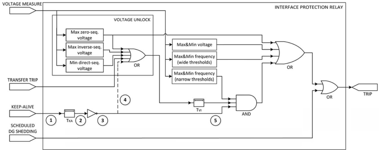
Figure 8. The logic implemented on Active Users' IPRs.
