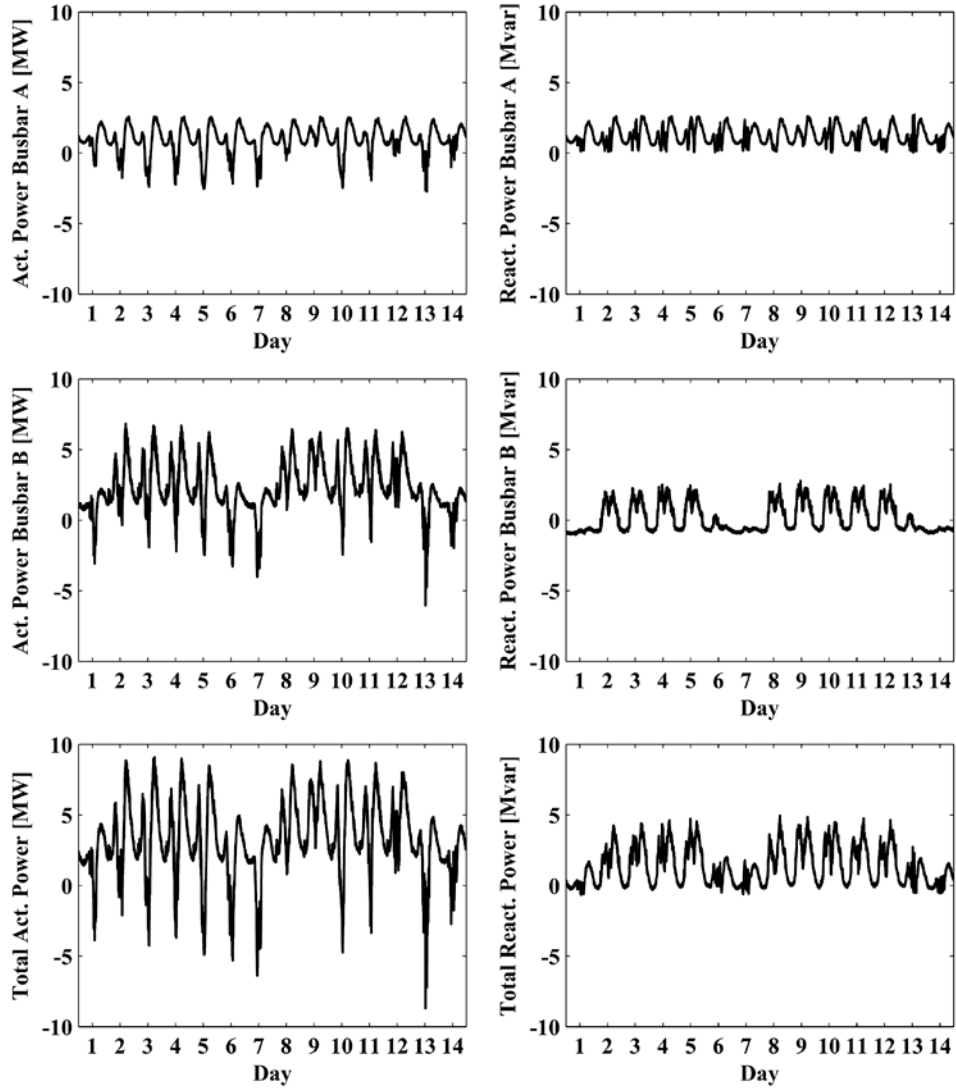
Figure 3. Active and reactive power withdrawals measured at the HV interface of the A.S.SE.M. substation during the period 6 - 19 January 2014.
