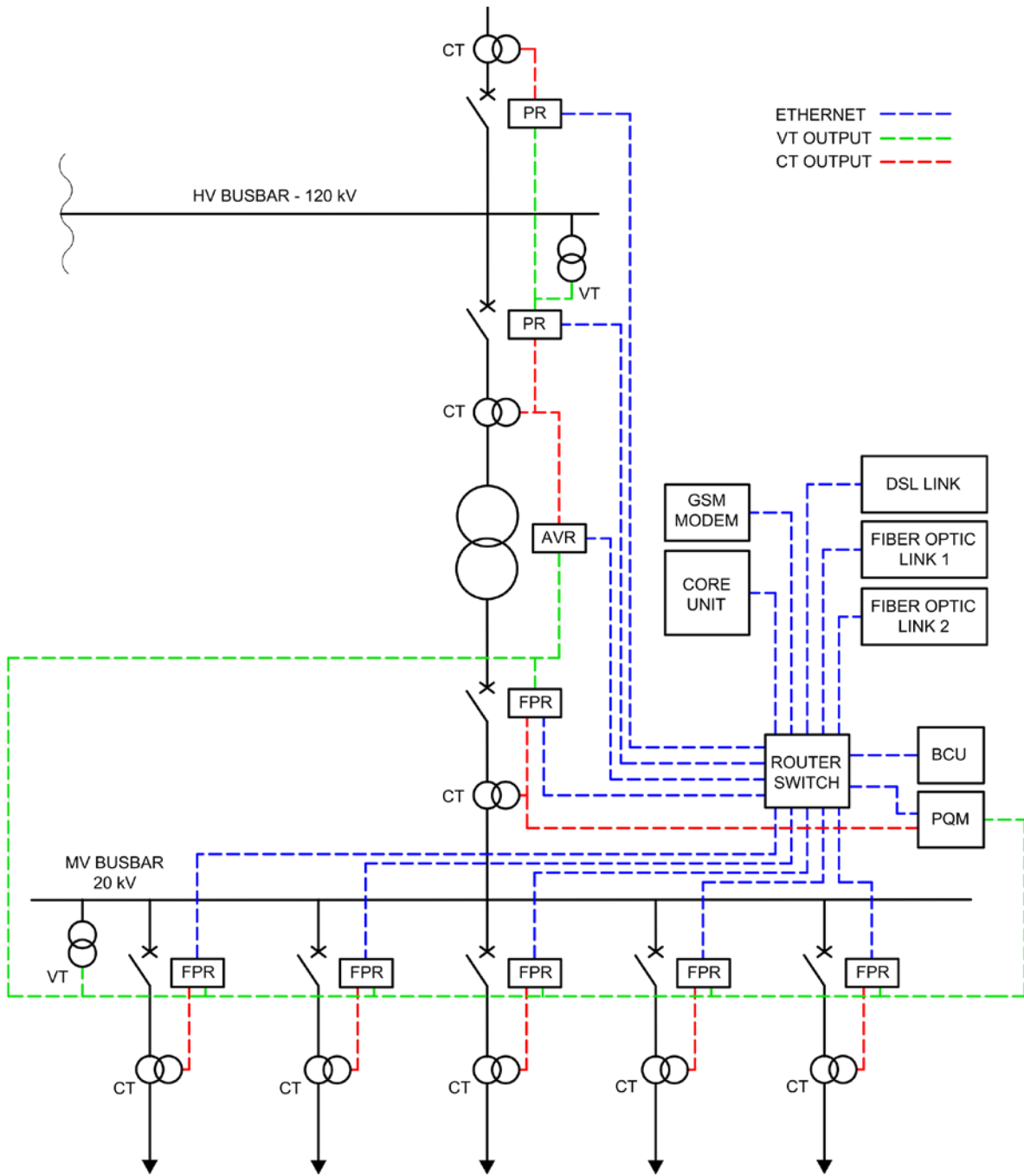
Figure 4. Functional architecture of the Smart Grid system for a MV busbar of the HV/MV substation.
