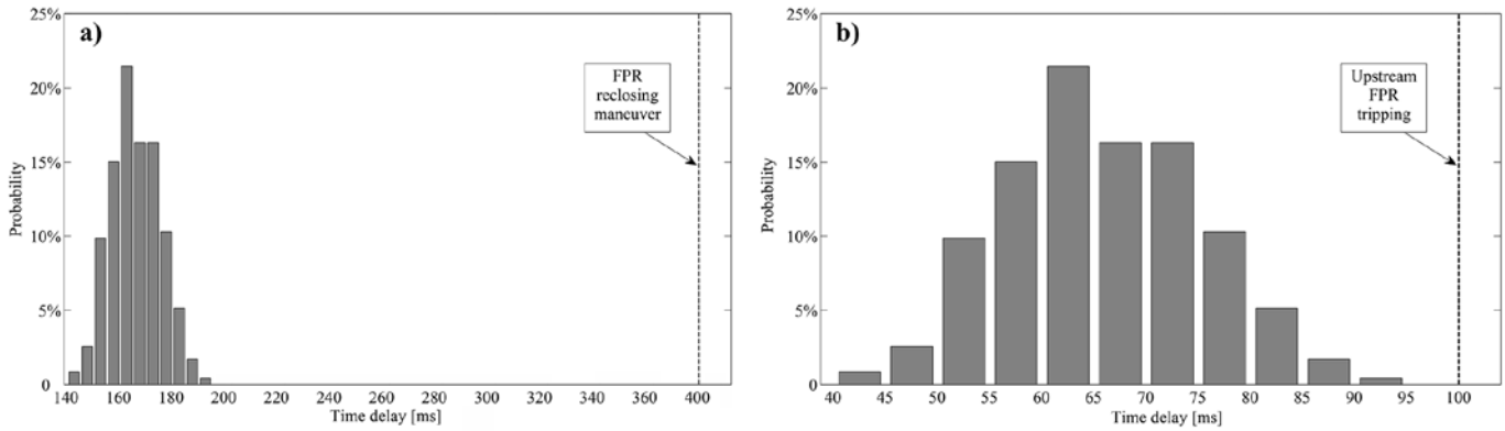
Figure 11. Estimated time for the IPR tripping (a) and the FPR inhibition (b).
