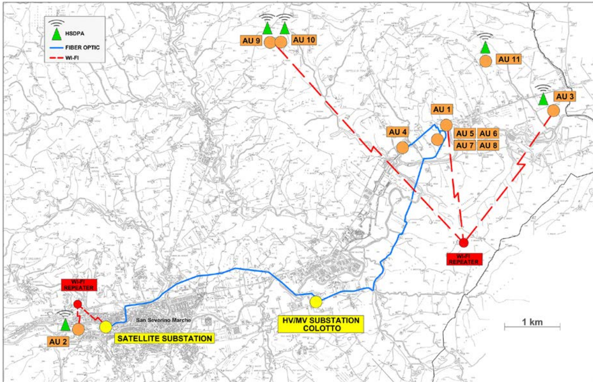
Figure 2. Communication system of the SG project.
