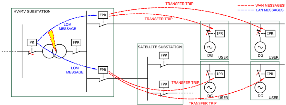
Figure 7. Transfer trip message in case of tripping of a HV protection relay.
