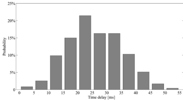
Figure 10. Probability density function of the time delay for the transmission of GOOSE messages.
