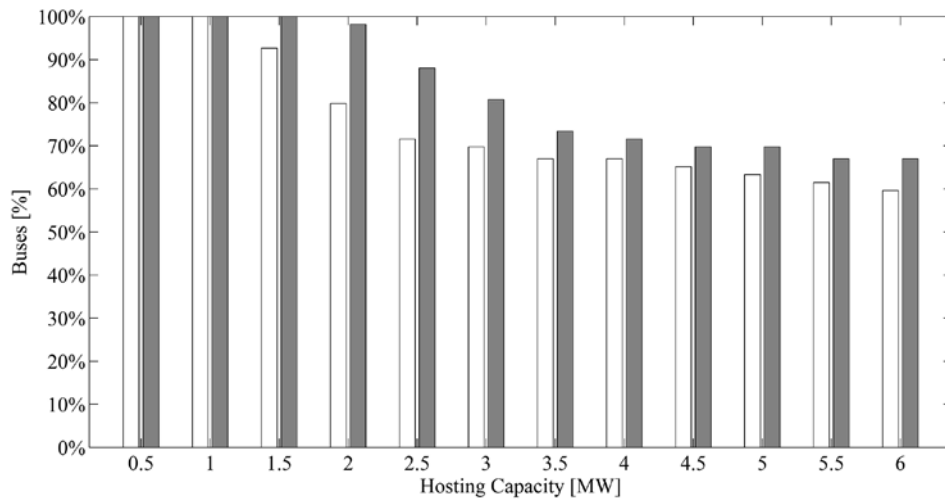
Figure 13. Nodal Hosting Capacity on the MV grid before (white) and after (gray) the SG project.
