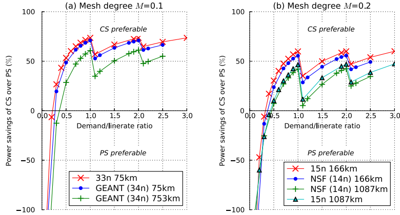
Fig. 5. Influence of the average physical link length on the relative savings of CS over PS (linerate = 10G). Longer link lengths result in lower savings, and explain why the savings profile of topologies such as Géant (average physical link length = 753 km) does not correspond very well with our artificial topology of the same node count but much shorter link length.
