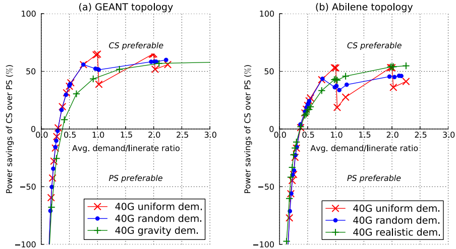
Fig. 8. Influence of different demand types on the savings of CS over PS, both for the (a) Géant and (b) Abilene topology (linerate = 40G). While uniform demands show a distinct stepwise behavior, more realistic demand sets (i.e., random and gravity demands) smooth out this behavior.
