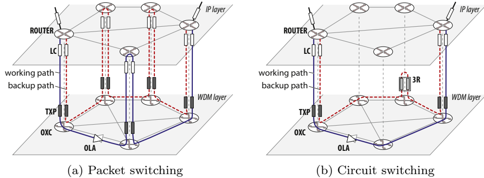
Fig. 1. The packet-switched and circuit-switched network architectures considered in this paper, showing both the bidirectional working path (solid lines) and backup path (dashed lines) under a 1 + 1 protection scheme. (LC = Line Card, TXP = Transponder, OXC = Optical Cross-Connect, OLA = Optical Line Amplifier, 3R = 3R regenerator.)
