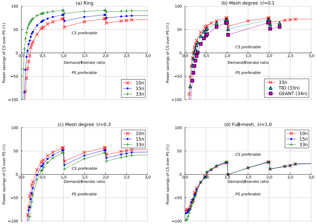
Fig. 4. Influence of the node count on the power savings of CS over PS (for linerate = 40G). Only for sparse topologies (i.e., (a)–(c)) the node count has an influence on the savings. While for a ring topology a higher node count leads to more savings, this is not consistently the case for other sparsely meshed topologies. The relatively large deviation of the Géant topology from the general trend is explained in Fig. 5.
