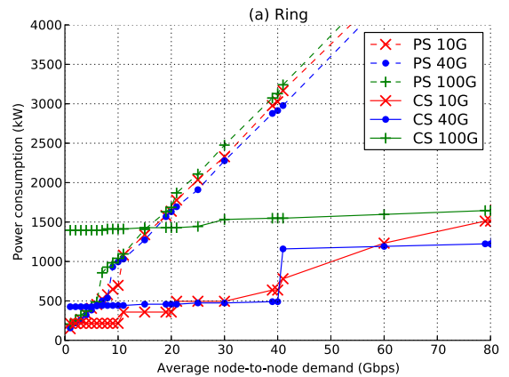
Fig. 9. Influence of using more accurate IP power consumption modeling on the total power consumption (15-node topology). The overall shape of the curves is not affected; compare with Fig. 2(a).
