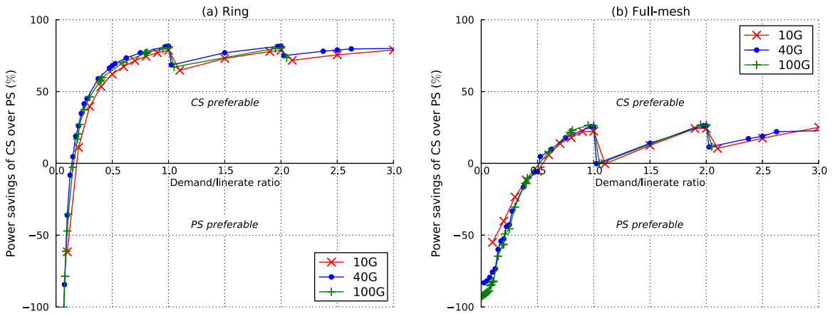
Fig. 3. Power savings of CS over PS mapped to the ratio of the demand bitrate over the channel linerate (15-node topology). The savings show a stepwise behavior around integral multiples of this ratio (i.e., the savings suddenly drop when the node-to-node traffic demands surpass the channel linerate). The ratio's transition window where CS becomes more preferable than PS is relatively small and relatively independent of the channel linerate (especially for highly-meshed networks, where it is fixed at 1/2).
