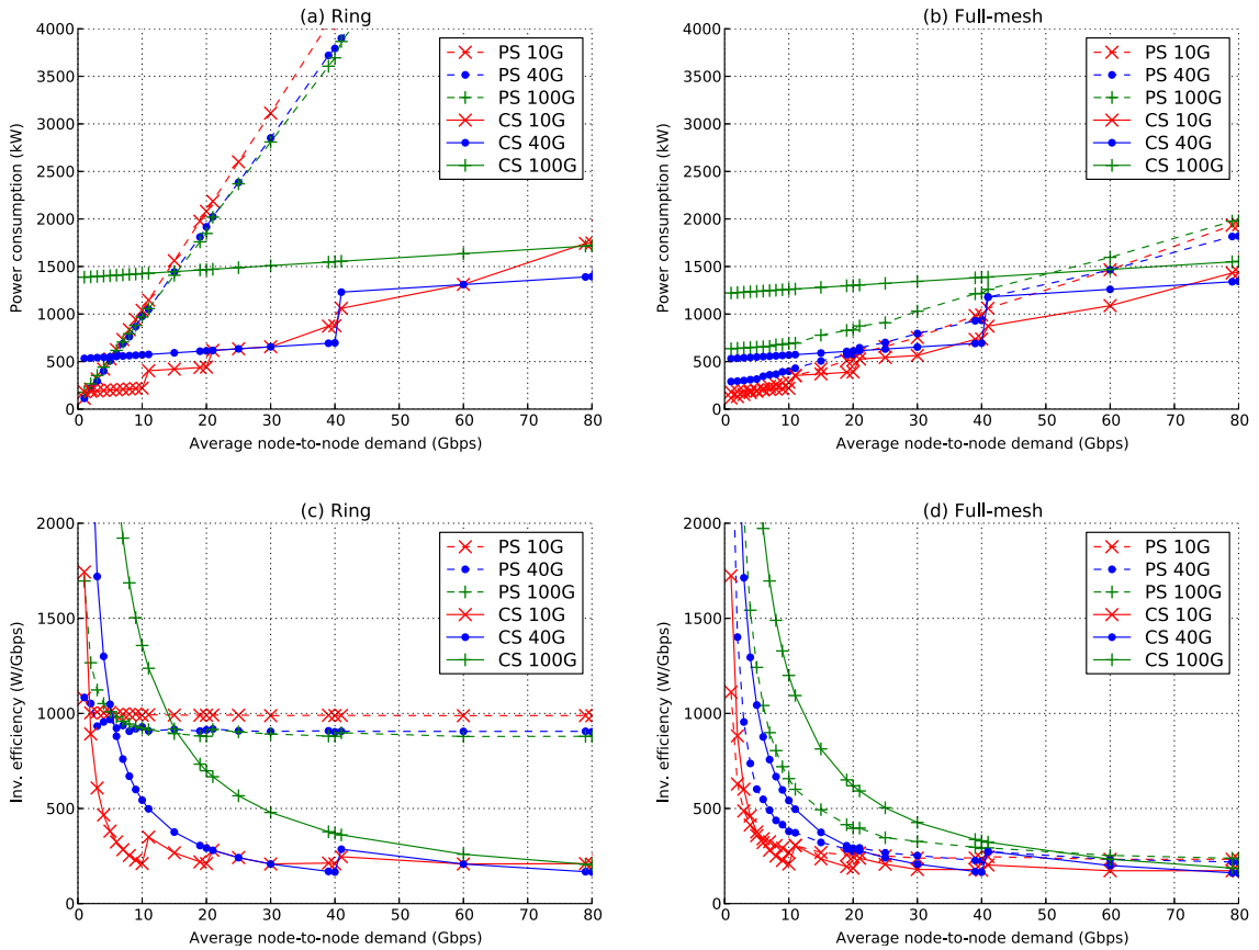
Fig. 2. The total power consumption and inverse power efficiency of a 15-node ring and full-mesh topology with increasing node-to-node traffic demand. The packet-switched (PS) paradigm shows an overall linear behavior, whereas the circuit-switched (CS) paradigm shows a stepwise behavior whenever the traffic demand becomes a multiple of the channel capacity. The power efficiency of PS in sparsely-connected networks is almost independent of the traffic demand, whereas for CS the power efficiency improves with increasing traffic.
