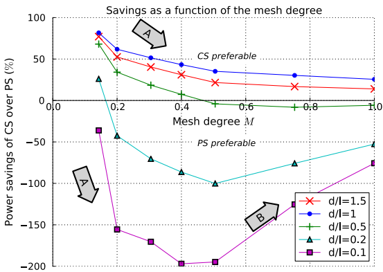
Fig. 7. Influence of the mesh degree and the demand/linerate ratio d/l on the relative savings of CS over PS (for \text{linerate} = 40\text{G} , and 15-node topologies). For low demand/linerate ratios there is an optimum point where PS is favorable. Effect A: the PS power consumption decreases with increasing mesh degree, as fewer IP hops are required. Effect B: the PS power consumption increases towards that of the CS solution, because the PS grooming potential decreases with increasing mesh degree.
