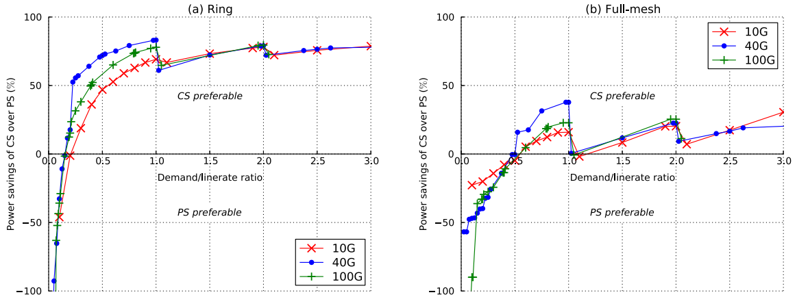
Fig. 10. Influence of using more accurate IP power consumption modeling on the power savings of CS over PS (15-node topology). The overall shape of the curves is not affected; compare with Fig. 3.
