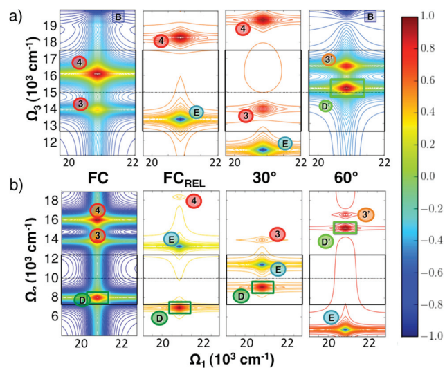
Fig. 14 Simulated 2D (xxxx) spectra for the two-colours 2DVis (a) and the two-colour 2DVis/NIR (a) setups. 2D spectra are reported for the selected MEP point from the FC to the 60^\circ structure. The complex part of the combined rephasing and non-rephasing (KI + KII) signals is plotted on a logarithmic scale. The peaks are labelled according to the transition assignment in Fig. 13. Black boxes indicate the used 5000 \text{ cm}^{-1} bandwidth and central frequencies are indicated with dotted lines. Reproduced from ref. 99.
