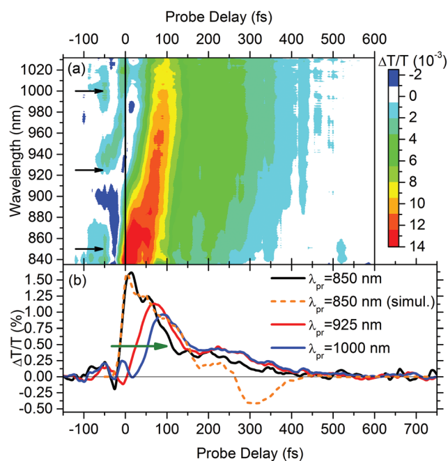
Fig. 10 (a) \Delta T/T map of isoRh in the NIR range, following excitation by a 10 fs pulse at 500 nm; (b) solid lines: time traces at selected probe wavelengths; dashed line: MD-simulated trace at 850 nm. The green arrow highlights the delayed formation of the SE for longer wavelengths. Adapted from ref. 94.
