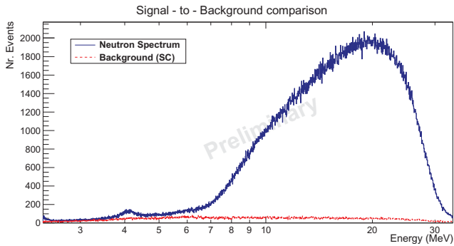
FIG. 3. Comparison of the measured neutron spectrum without (solid blue) and with (dashed red) the shadow cones (SC), to estimate the scattered neutrons background.
