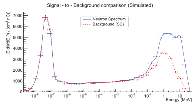
FIG. 2. Comparison of the FLUKA simulated neutron spectrum without (solid blue) and with (dashed red) the shadow cones (SC), to estimate the scattered neutrons background.
