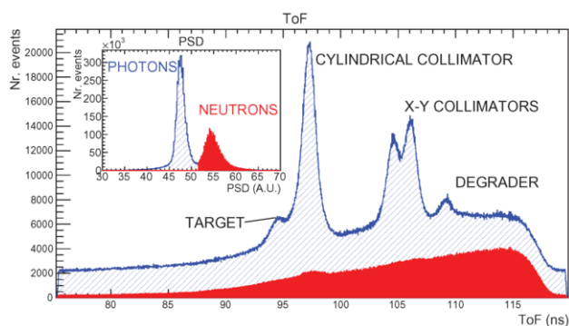
FIG. 1. Raw TOF spectrum. The PSD spectrum in the inset shows the separation between neutrons (solid red) and photons (hatched blue). The peaks in the photon spectrum correspond to production in the beam-line elements. The reduction of the gamma background is evident in the TOF spectrum.
