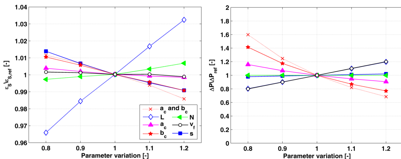
Figure 6. Parametric analysis of sensible effectiveness and pressure drop. (Reference conditions: a_c = 2 mm, b_c = 2 mm, s = 0.06 mm, L = 0.2 m, v_f = 1.5 m·s -1 , N = 10 rev·min -1 , T_{su,in} = 10 °C, T_{ex,in} = 30 °C, X_{su,in} = 3.7 g·kg -1 , X_{ex,in} = 7.7 g·kg -1 , \varphi_{su,in} = 50\% and \varphi_{ex,in} = 30\% ).
