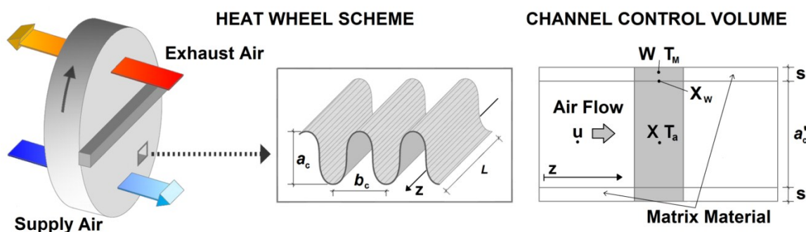
Figure 1. Scheme of heat wheel and channel control volume.
