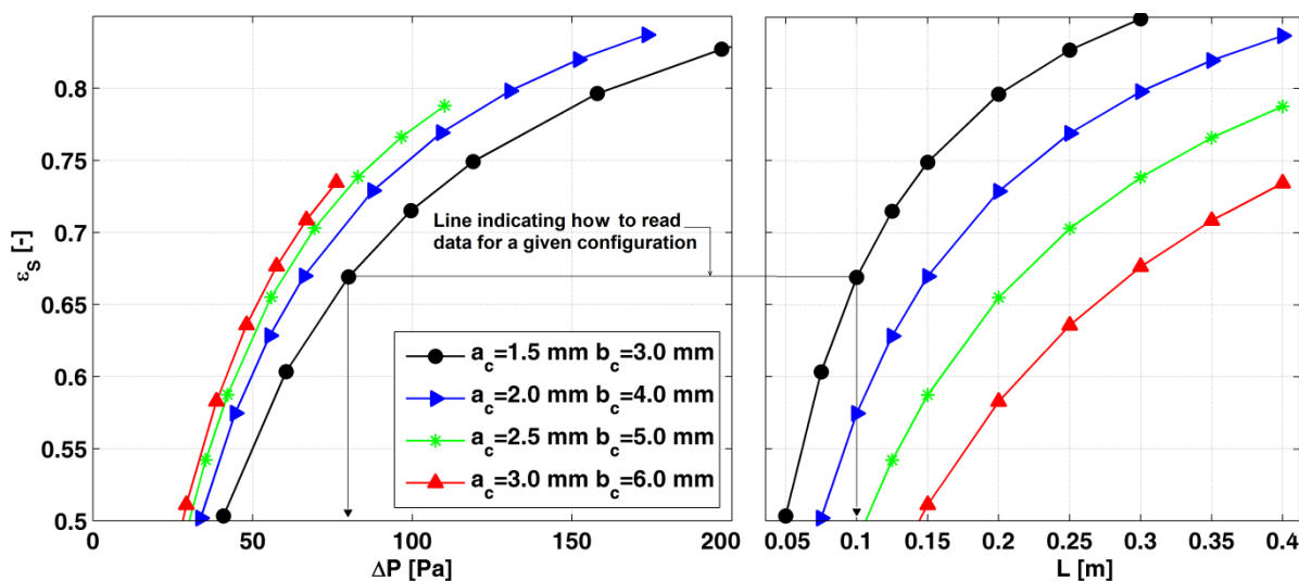
Figure 9. Optimal wheel configurations at constant channel aspect ratio b_c/a_c=2 and at v_f = 2.5 m·s -1 for different length ( T_{su,in} = 10 °C, T_{ex,in} = 30 °C, X_{su,in} = 3.7 g·kg -1 , X_{ex,in} = 7.7 g kg -1 , \varphi_{su,in} = 50\% , \varphi_{ex,in} = 30\% , s = 0.05 mm and N = 10 rev·min -1 ).
