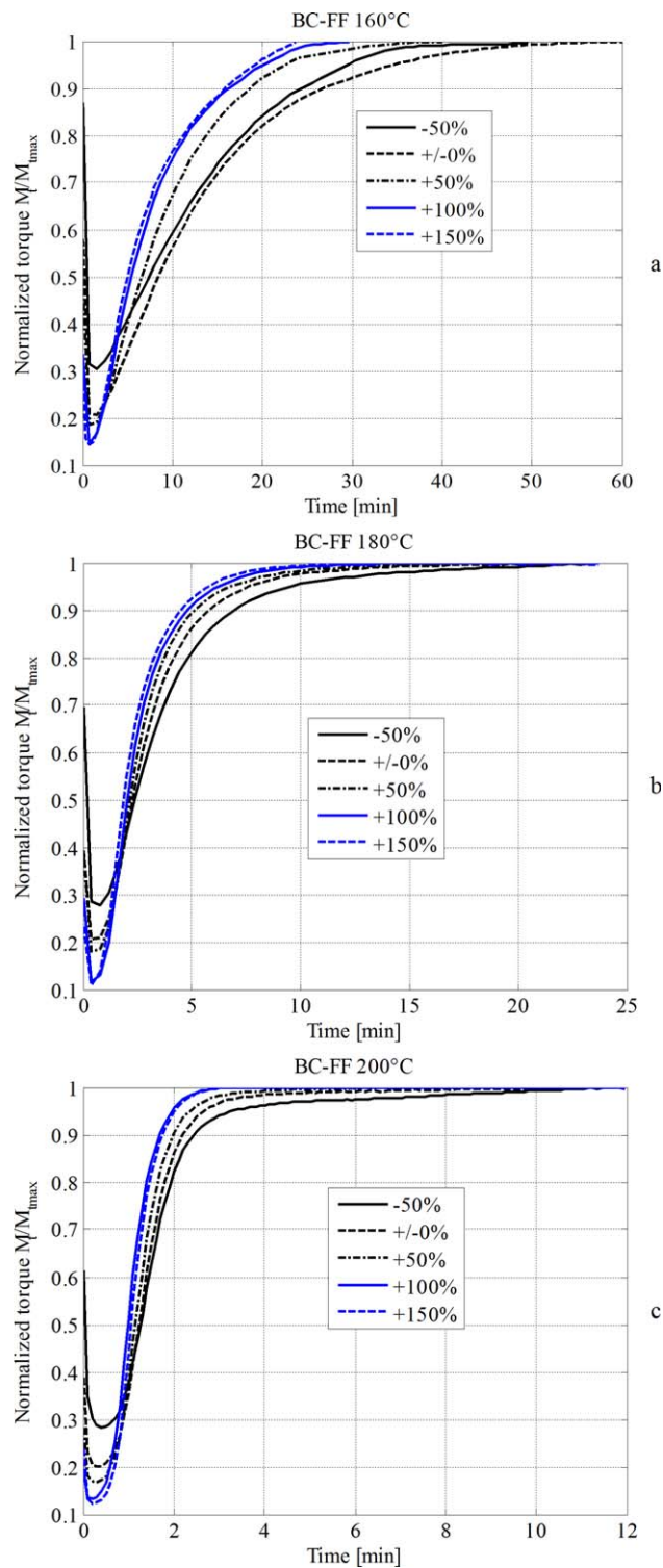
Figure 8. BC-FF peroxide. Normalized experimental rheometer curves at different peroxide concentrations. a: 160°C, b: 180°C, c: 200°C. [Color figure can be viewed in the online issue, which is available at wileyonlinelibrary.com .]
