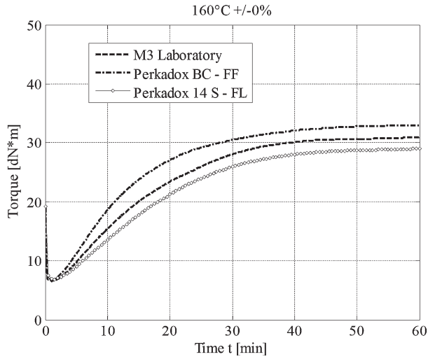
Figure 3. Experimental torque curves at \pm 0\% concentrations. a: 200^{\circ}\text{C} , b: 180^{\circ}\text{C} , c: 160^{\circ}\text{C} .
