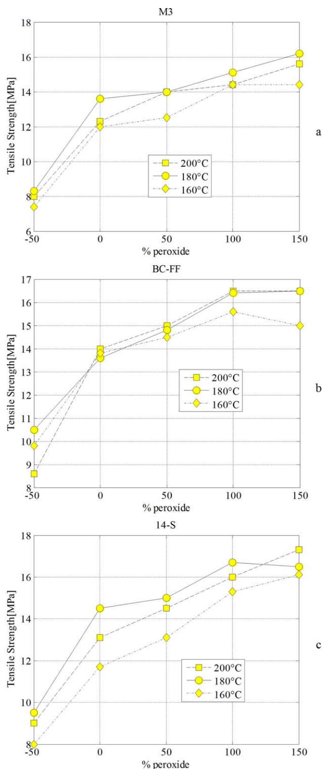
Figure 15. Tensile strength experimental results as a function of peroxide concentration. a: M3, b: BC-FF, c: 14-S. [Color figure can be viewed in the online issue, which is available at www.interscience.wiley.com .]
