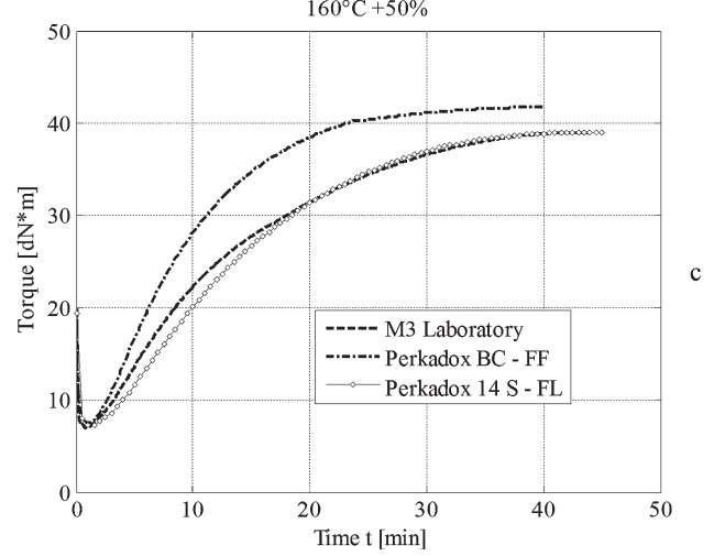
Figure 4. Experimental torque curves at +50\% concentrations. a: 200^{\circ}\text{C} , b: 180^{\circ}\text{C} , c: 160^{\circ}\text{C} .
