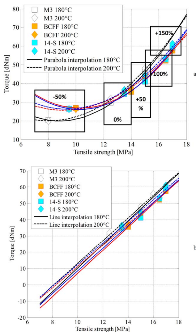
Figure 14. Tensile strength versus torque. a: Experimental data (points) and parabolic numerical interpolation. b: linear interpolation excluding –50% results. [Color figure can be viewed in the online issue, which is available at wileyonlinelibrary.com .]
