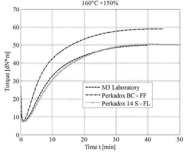
Figure 6. Experimental torque curves at 150% concentrations. a: 200°C, b: 180°C, c: 160°C.
