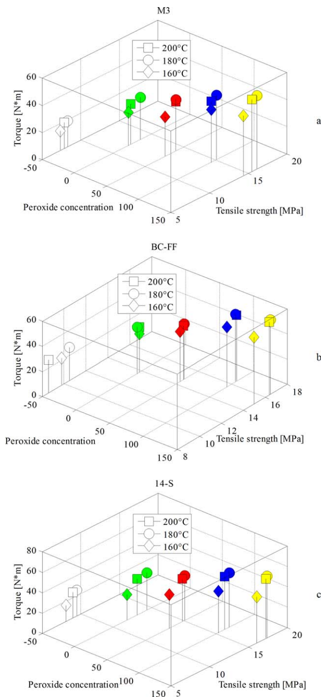
Figure 18. Experimental tensile strength-torque-% peroxide concentration diagrams as a function of vulcanization temperature. a: M3, b: BC-FF, c: 14-S. [Color figure can be viewed in the online issue, which is available at wileyonlinelibrary.com .]
