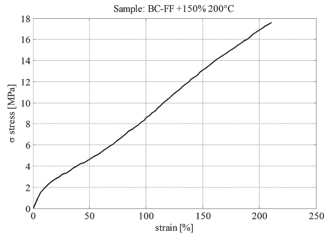
Figure 11. Typical stress–strain curve obtained experimentally on a vulcanized sample.
