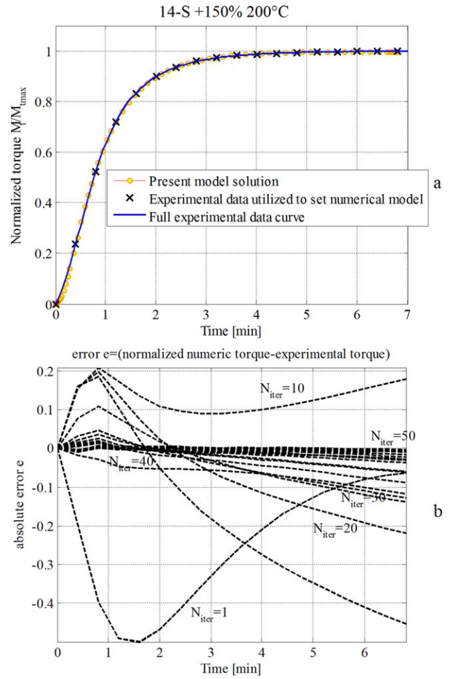
Figure 27. 14-S curing agent, 200°C. Comparison between experimental data and numerical model. a: full normalized curve, b: difference between numerical model and experimental normalized torque. [Color figure can be viewed in the online issue, which is available at wileyonlinelibrary.com .]
