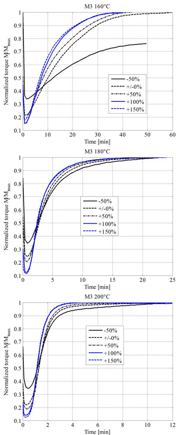
Figure 7. M3 peroxide mixture. Normalized experimental rheometer curves at different peroxide concentrations. a: 160°C, b: 180°C, c: 200°C. [Color figure can be viewed in the online issue, which is available at wileyonlinelibrary.com .]
