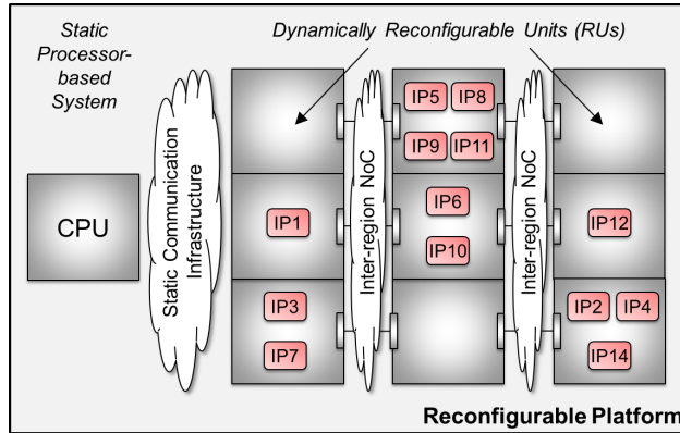
Fig. 1. The target hardware architecture
