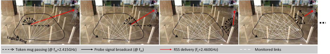
Fig. 4. Network architecture for device-free localization: timed-token beacon message passing.
