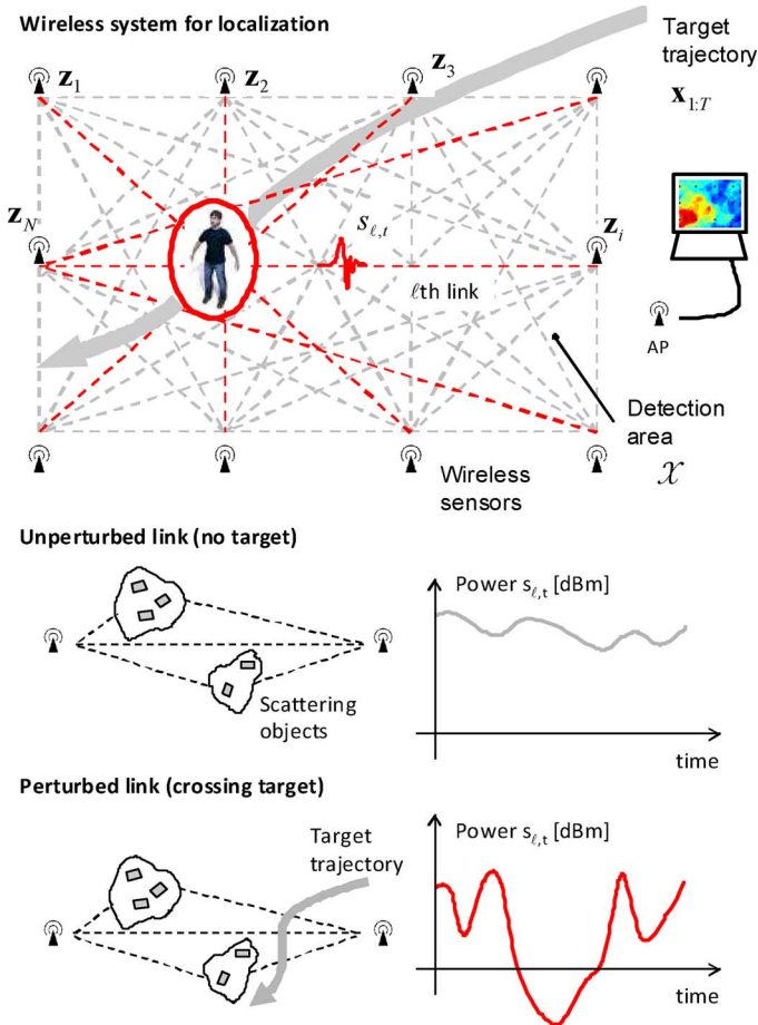
Fig. 1. Wireless infrastructure for device-free localization (top). Received signal power over the \ell th link due to the moving target (bottom figure).
