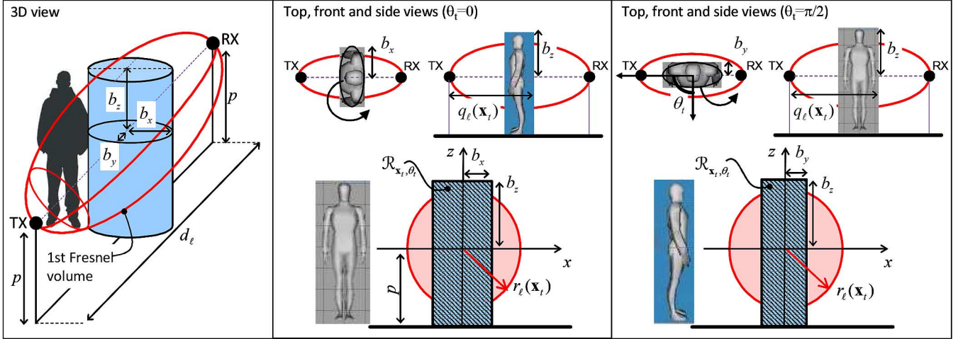
Fig. 2. Diffraction-based model for target object (human body scattering).
