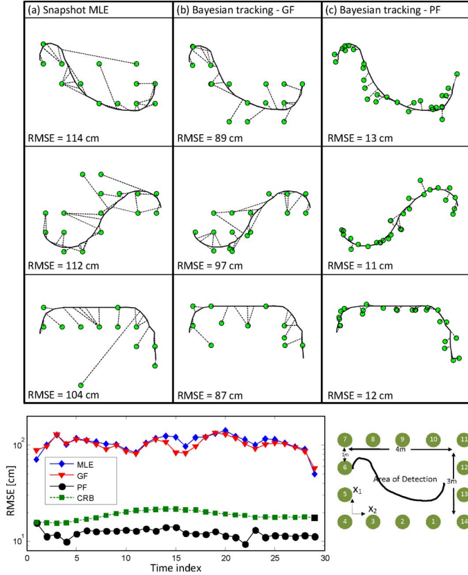
Fig. 9. Top figure: examples of location trajectories (solid lines) and related estimates (markers). From left to right: MLE, GF and PF based Bayesian tracking. Dashed lines connecting the true and estimated positions highlight the localization errors. The RMSE averaged over the trajectory is indicated for each case. Bottom figure: RMSE and CRB performance as a function of the position along the corresponding trajectory (indicated in the sub-figure).
