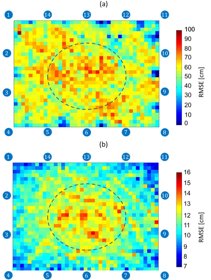
Fig. 10. RMSE for MLE (a) and PF Bayesian tracking (b) as a function of the target position within the detection area \mathcal{X} . (a) MLE. (b) PF Bayesian tracking.
