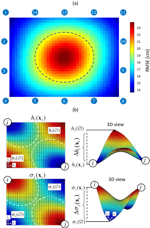
Fig. 6. (a) CRB on the location estimate accuracy (expressed in cm) for the square network deployment; (b) Attenuation and standard deviation analytical maps for the single link (i, j) based on the diffraction model. (a) CRB to positioning accuracy. (b) Attenuation and standard deviation maps.
