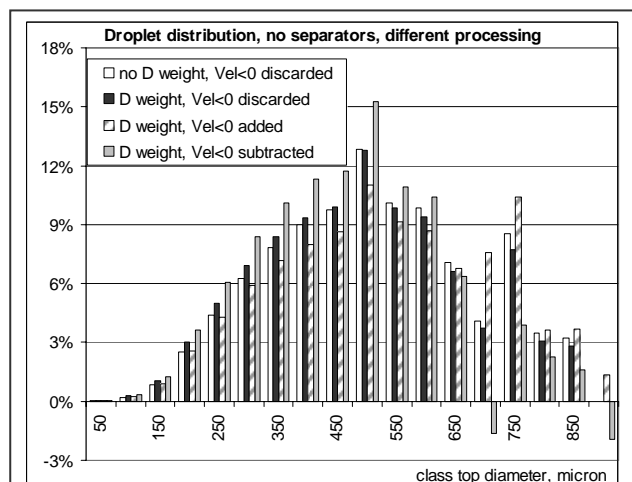
Figure 8 Droplet volume distribution, without separators, processed with four different procedures.
