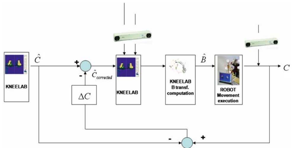
Fig. 3 Update of matrix C if an error between the desired mask position and orientation and the actual ones, with reference to the anatomical DRB, is detected by the localization system
