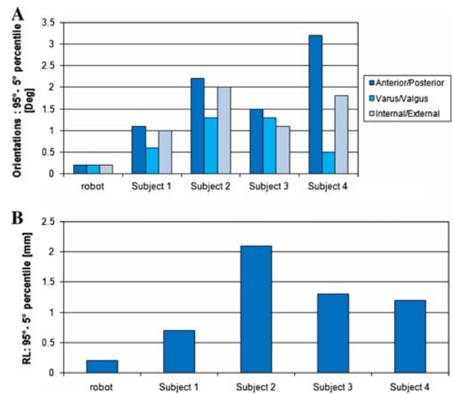
Fig. 7 Stability in the orienting (a) and in the positioning (b) of the cutting mask
