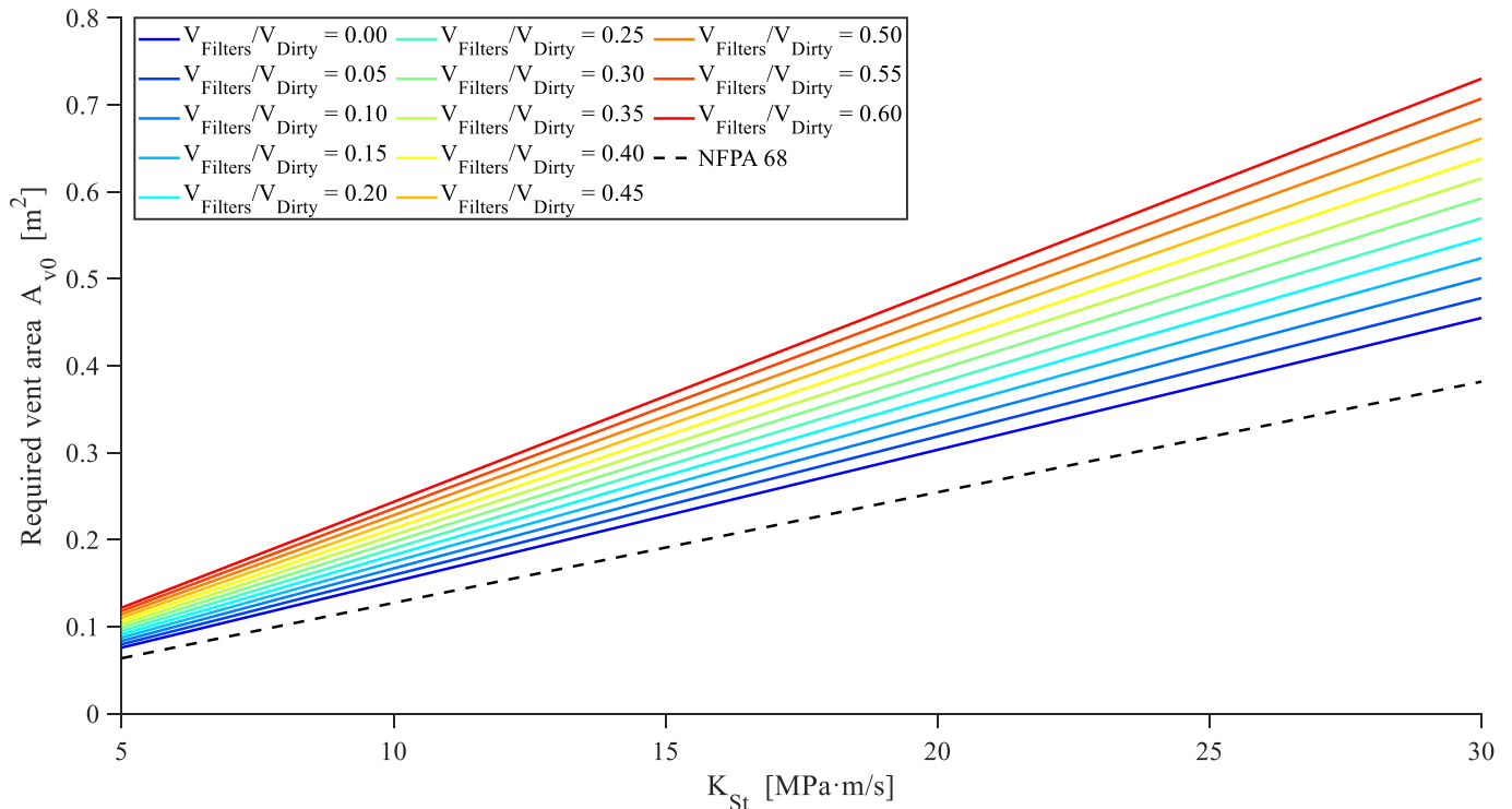
Fig. 12. Required vent area, A_{V,0} , versus effective deflagration index K_{St} for V_{Filters}/V_{Dirty} = 0.00 to V_{Filters}/V_{Dirty} = 0.60 . The proposed correlation converges with the NFPA 68 vent sizing in the absence of internal obstruction.
