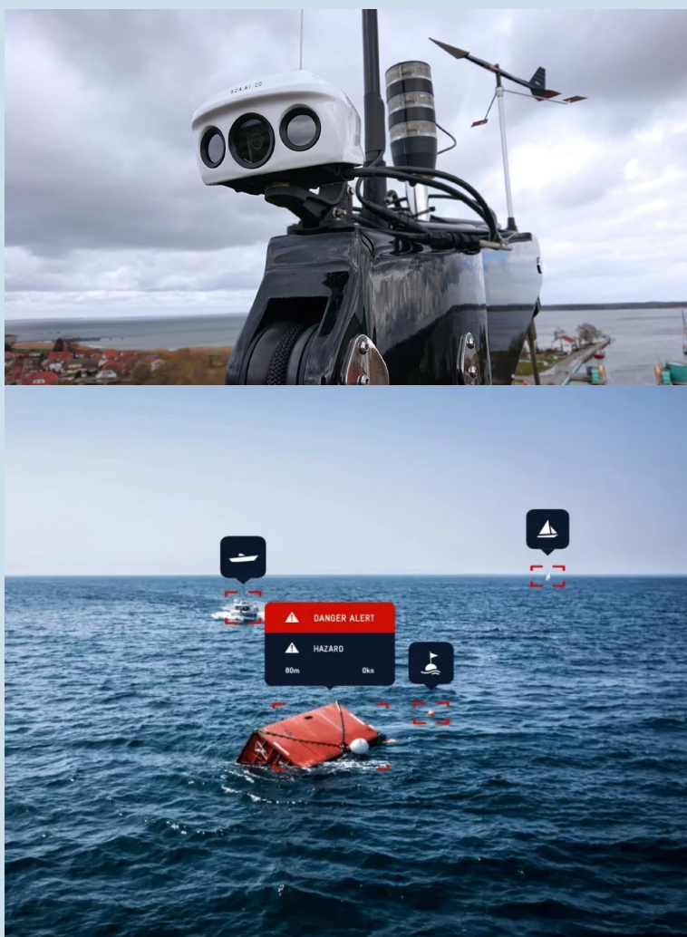
Figure 13. SEA.AI equipment at the top of a racing sailingboat, and its reported images in AR. Credits: SEA.AI.
