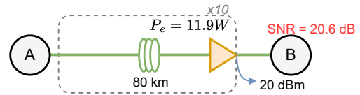
B) Beyond SoTA HCF optical communication system
