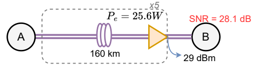
Fig. 1: Illustrative example of an SSMF (10 x 80 km spans) and an HCF (5 x 160 km spans) optical communication system
