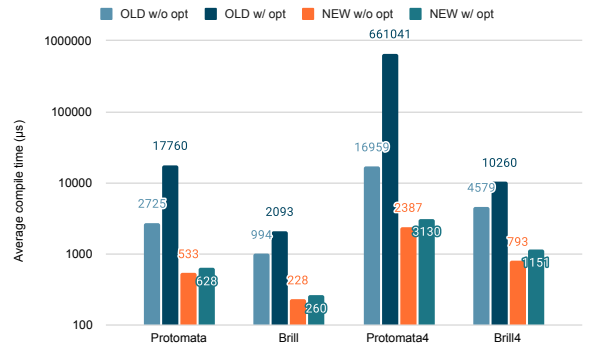
Figure 9. Compilation time comparison (log scale) of the new and old compilers w/ and w/o optimizations.
