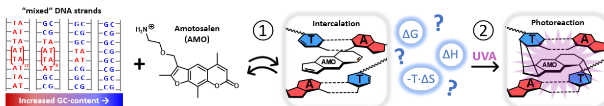
Figure 4: Interaction of amotosalen (AMO) and different “mixed” DNA oligomers. ① Reversible intercalation reaction. ② UVA-induced covalently linked interstrand cross-links with thymine bases. Here, the recently found unique capacity of AMO to intercalate preferentially into long AT-DNA strands, compared to short GC-strands [6], is explored by means of Isothermal Titration Calorimetry (ITC) in combination with Molecular Dynamics Simulations and Molecular Docking . A favourable free binding energy in AT-intercalation sites might lead to a higher cytotoxicity of new psoralen structures, evading the PET process [7]. Thus, quantification and optimization of the thermodynamics of intercalation might yield more efficient PUVA agents.
