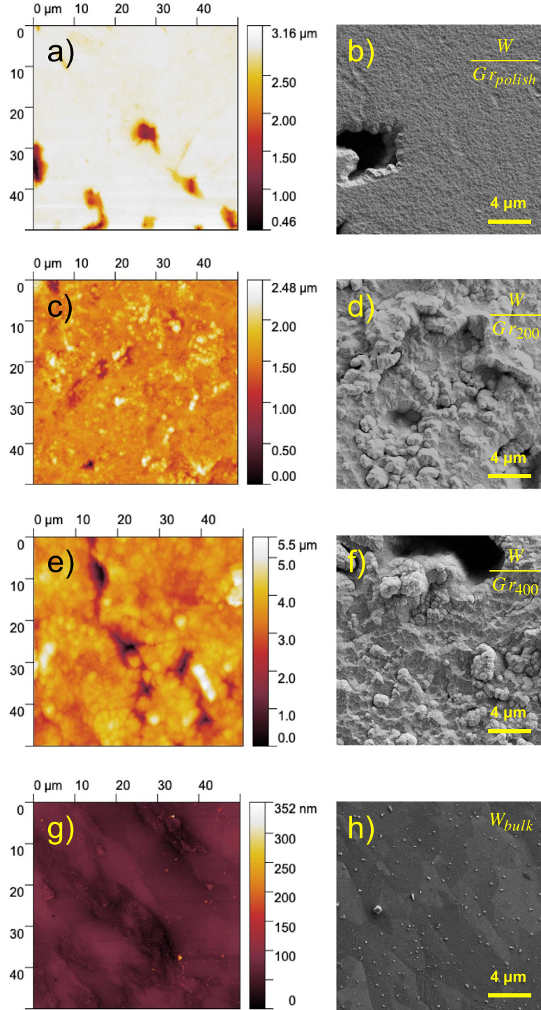
Figure 3. 50 \times 50 \mu\text{m}^2 AFM and SEM top-view images of the 500 nm thick W coating deposited on: polished graphite substrates (a), (b) and plasma-etched graphite substrates with R_a of 200 nm (c), (d) and 400 nm (e), (f). Micrographs of a bulk W sample are also included (g), (h).
