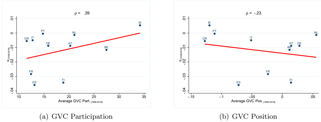
Figure 2: Global Value Chain and the Phillips Curve
