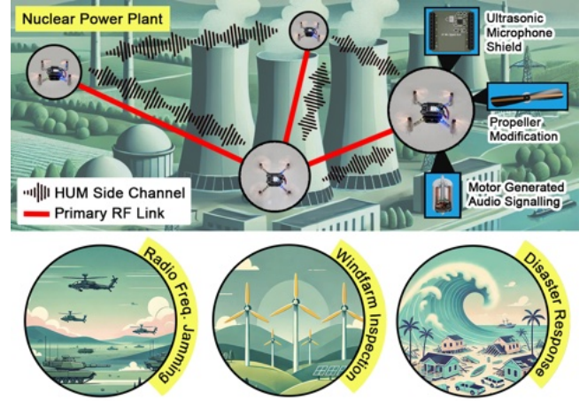
Figure 1: HUM communication: we use motors as transmitters, custom changes to existing propellers to reduce interference noise, an ultrasonic microphone at the receiver, and a dedicated communication protocol. A demonstration video can be found online: https://youtu.be/Ji_CjWFnaB4
