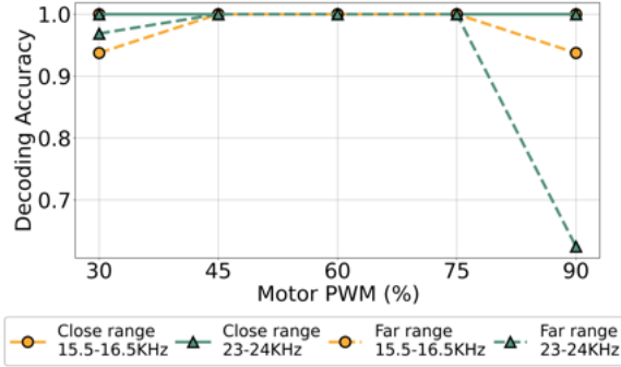
Figure 19: HUM decoding accuracy with varying PWM percentage of the HUM transmitting drone.
