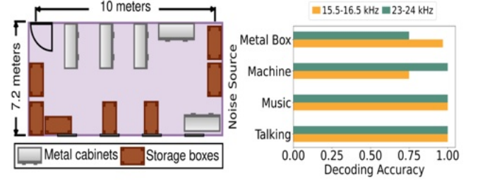
Figure 20: Floor map of the HUM communication test environment with metallic obstacles (left) and decoding accuracy with different ambient noise sources (right).
