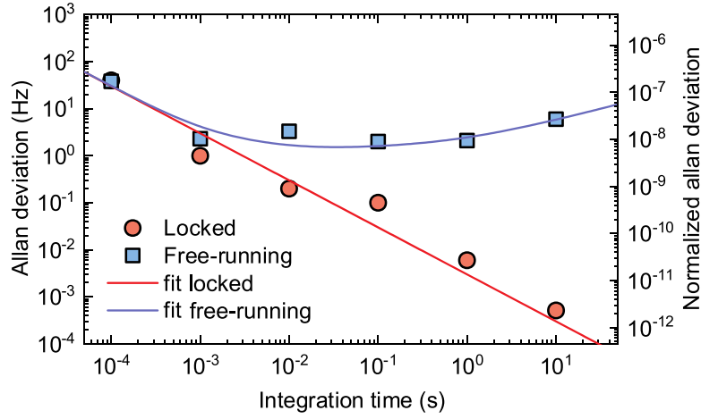
Fig. 5. Allan variance of the pulse repetition frequency in free-running and in locked conditions, respectively. Continuous lines represent the best curve fittings: \sigma(\tau)_{\Delta\nu} = (5 \times 10^{-6} \tau^{-1} + 2 + 3\tau)^{1/2} and \sigma(\tau)_{\Delta\nu} = 3 \times 10^{-3} \tau^{-1} in free-running and locked conditions, respectively.
