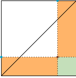
Figure 2: Partition of [0, 1]^2 as in the proof of Theorem 4.3.
