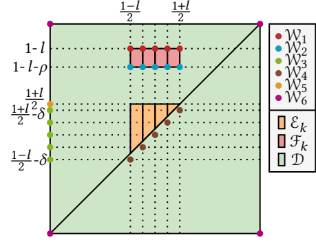
Figure 3: Representation of the support of the distributions \mu_k and their partitions.
