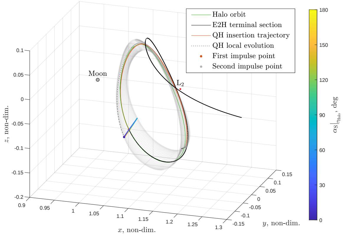
Figure 15: QH insertion phase for the most propulsively efficient Earth-to-QH transfer from the payload perspective. Corresponding E2H section is represented in Figure 7.
