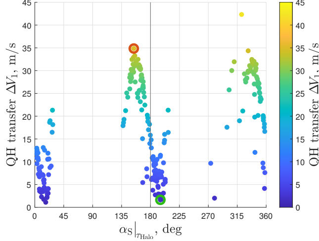
Figure 13: Cost of first impulse to insert into QH transfer as function of the initial solar angle.
