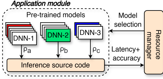
Fig. 6. Selecting quantized models for accuracy configuration of DNNs
