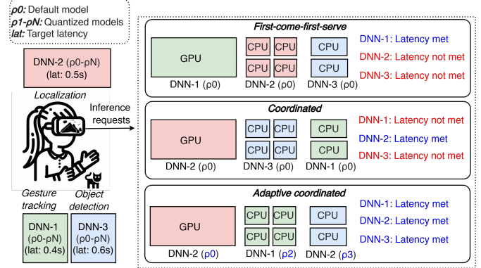
Fig. 1. Orchestrating concurrent DNNs with different scheduling strategies
