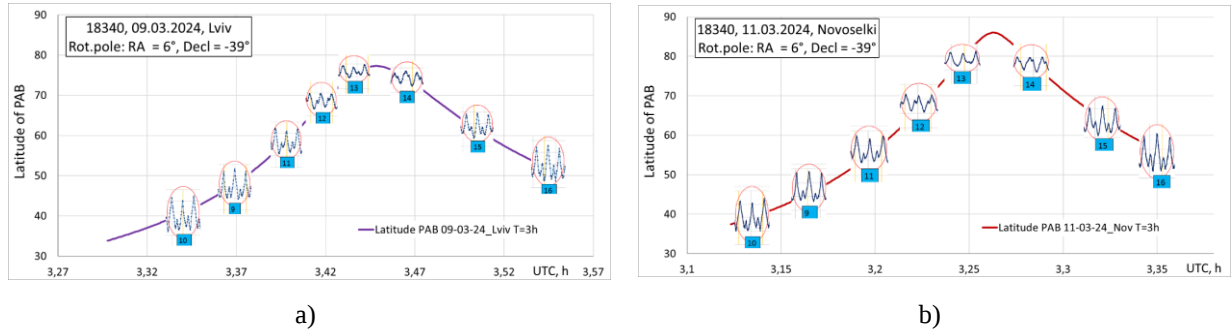
Fig. 17. Change in PAB's latitude for the pole of the rotation axis RA = 6^\circ , Decl = -39^\circ and the corresponding photometric patterns obtained during the passage of 18340: a) AO LNU on 09-03-2024; b) OEOS-2 (Novosilki) on 11-03-2024.
