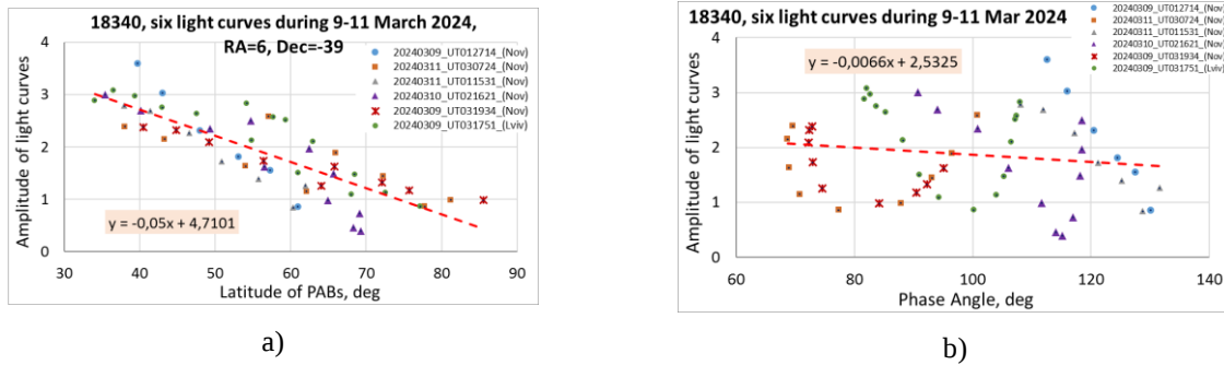
Fig. 18. Dependence of the LCs' amplitude on the latitude of PABs for six passes of the 18340 in the interval 09 – 11 March 2024 and the adopted direction of the rotation axis RA = 6^\circ , Decl = -39^\circ (a); Dependence of the LCs' amplitude on the phase angle (b).
