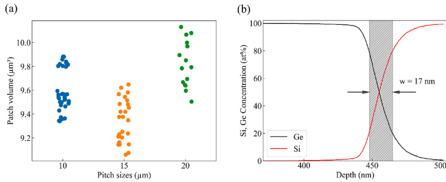
Fig. 4. (a) Volume (height \times area) of 5 \times 5 \mu\text{m}^2 patches on the 500 nm sample for different pitch sizes. (b) Si and Ge concentration at the Ge/Si heterointerface as measured by ToF-SIMS.
