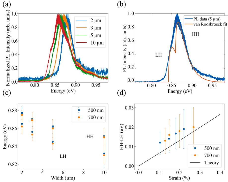
Fig. 10. (a) PL emission at 80K of a 700 nm sample normalized to unit height. (b) PL van Roosbroeck fitting of a spectrum from a patch of width 5 \mu\text{m} and thickness 700 nm. (c) Transition energy as a function of patch width. (d) HH-LH separation as a function of strain. The black line is a theoretical value calculated as described in the text.
