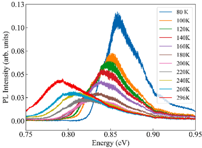
Fig. 11. Temperature dependence of PL spectra of a 10 \mu\text{m} patch with thickness 700 nm.
