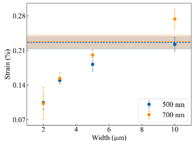
Fig. 6. Strain measured by Raman spectroscopy at the center of the patches, as a function of patch width for thickness (blue) 500 nm and (orange) 700 nm. Values are obtained from 9 points around the center of the patch, and reported as average and standard deviation. Dashed lines mark the strain value measured in the large SIMS control structures.
