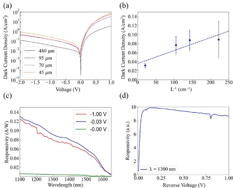
Fig. 12. (a) Dark current density as a function of the voltage for devices featuring lateral dimension of 480 μm (black line), 95 μm (purple line), 70 μm (red line) and 45 μm (orange line). (b) Dark current density as a function of the inverse of the lateral size of the photodiodes. (c) Responsivity at reverse bias voltages of 0V (green curve), 0.03 V (blue curve) and 1V (red curve) for one 480 μm photodiode. (d) Responsivity of the 480 μm device at \lambda = 1300 nm as a function of the reverse bias voltage.
