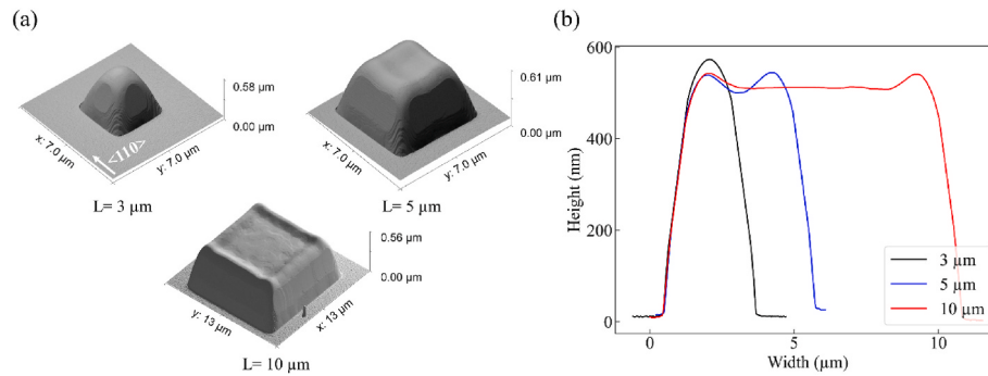
Fig. 2. (a) AFM 3D topography of 3, 5, 10 \mu\text{m} -wide patches. (b) Corresponding height profiles.
