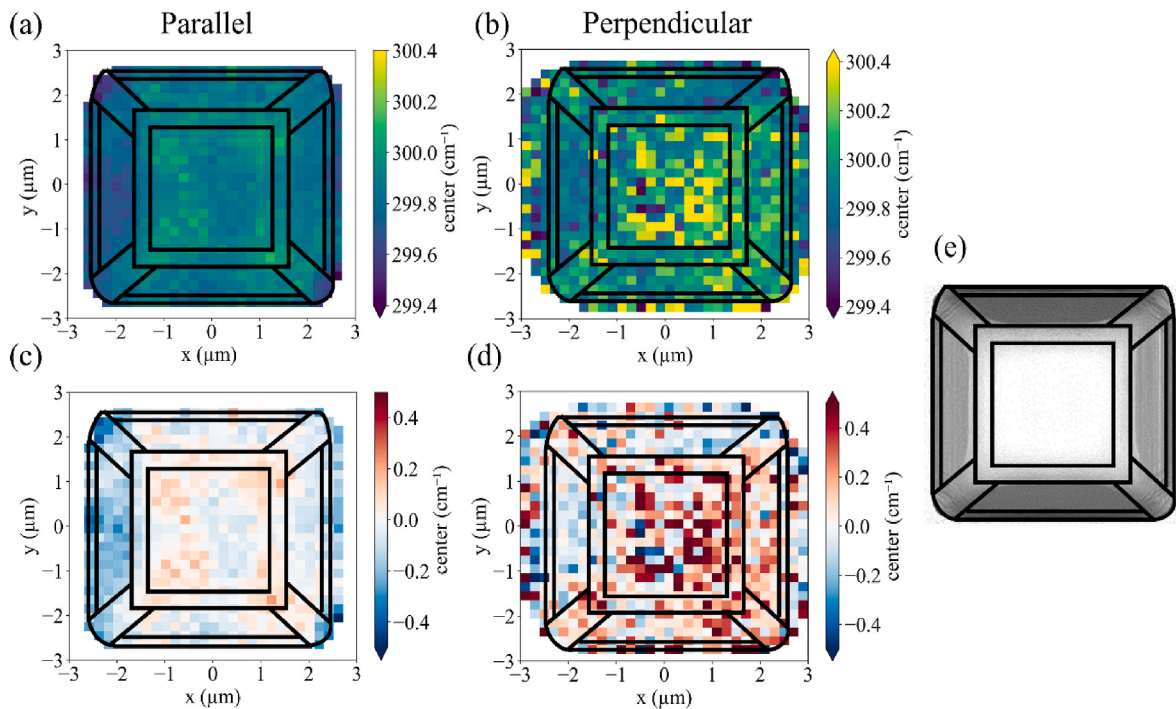
Fig. 8. (a) (b) Peak position from polarized Raman mapping of Ge 5 \times 5 \mu\text{m}^2 for parallel and perpendicular configuration. (c) (d) Map of the difference between the peak positions and the peak position in the center of the patch in parallel configuration. (e) AFM topography with marked facets.
