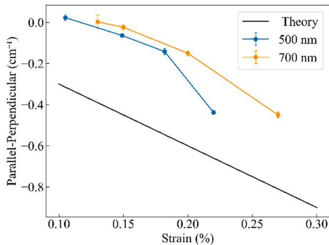
Fig. 9. Difference of the average peak position in the center of the maps in parallel and perpendicular configurations for different samples and patch size versus biaxial strain measured in the center. The black line is calculated as described in the text.
