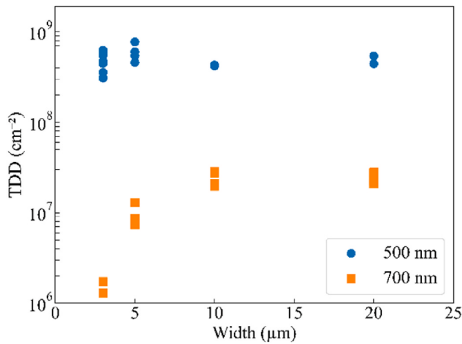
Fig. 5. TDD in patches of different width with thickness (blue) 500 nm and (orange) 700 nm.
