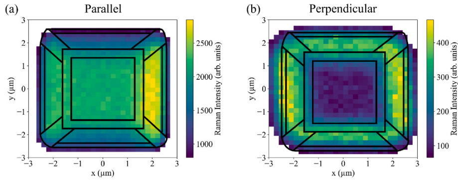
Fig. 7. Polarized Raman mapping with facet distribution of a 5 \times 5 \mu\text{m}^2 patch with thickness 700 nm. Intensity of (a) parallel and (b) perpendicular configuration; the left right asymmetry of the measured intensities can be the effect of substrate tilt during measurements. Black lines outline the facets of the patch as measured by AFM.
