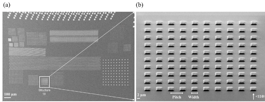
Fig. 1. (a) SEM plan view of a SEG Ge sample, with various patches arrays. (b) Magnification of Ge patch of 5 \times 5 \mu\text{m}^2 . Definition of Pitch and Width are marked.
