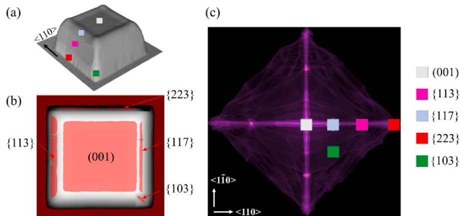
Fig. 3. (a) Identification of facets on AFM 3D topography of a 10 \times 10 \mu\text{m}^2 patch on the 500 nm sample for different pitch sizes. (b) Faceting distribution for 10 \times 10 \mu\text{m}^2 patch. (c) Angular distribution of the facet from AFM analysis.
