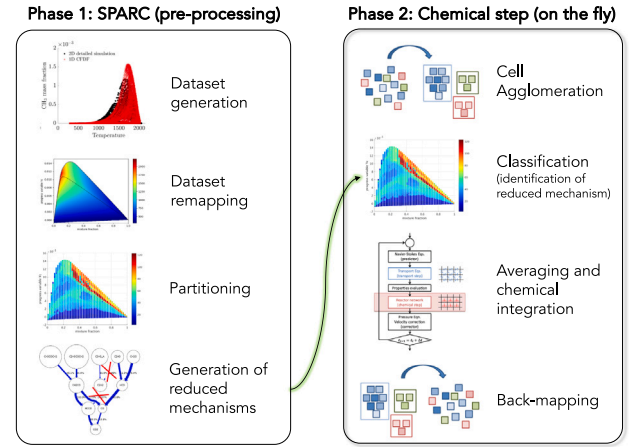
Fig. 1. Tabulation-based sample-partitioning adaptive reduced chemistry and cell agglomeration methodology.
