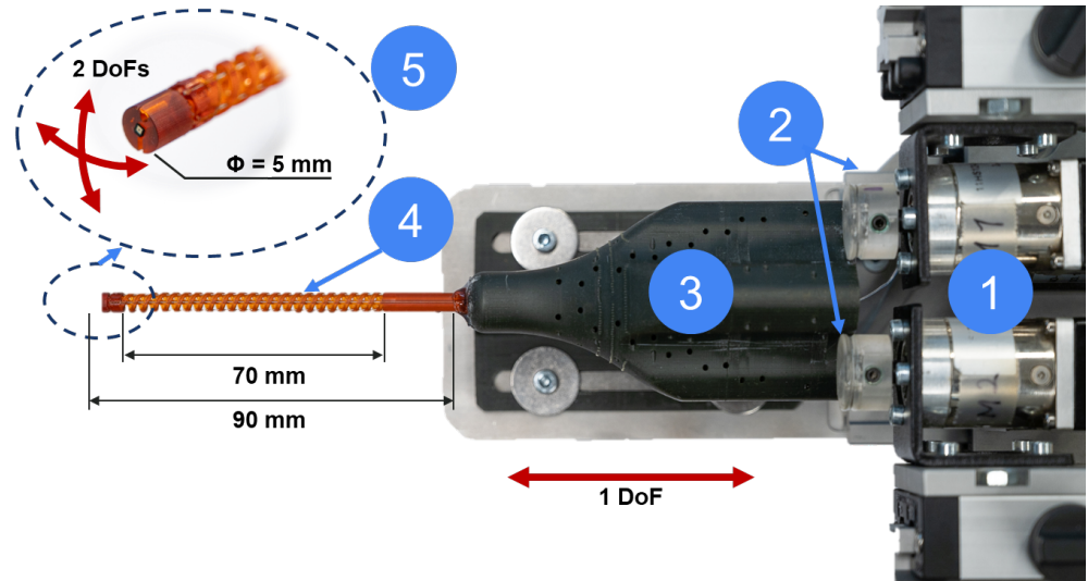
Figure 1. The robotic endoscope system, ATLAScope, to simulate a robotized ureteroscopy. (1) Two stepper motors; (2) two pulleys; (3) cable tunnels to guide driving cables; (4) soft robotic arm with HelicoFlex design, with a total length of 90 mm and a steerable segment of 70 mm; (5) miniaturized endoscopic camera and the two bending directions of the robotic arm.
