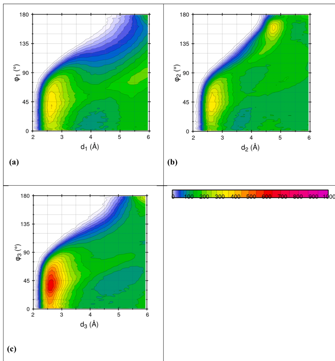
Fig. 9. Combined distribution functions for the angle C6-H3...O1 (a), C6-H3...O2 (b), and C6-H3...O3 (c) as functions of distances d_{H3-O1} , d_{H3-O2} , d_{H3-O3} , respectively.
